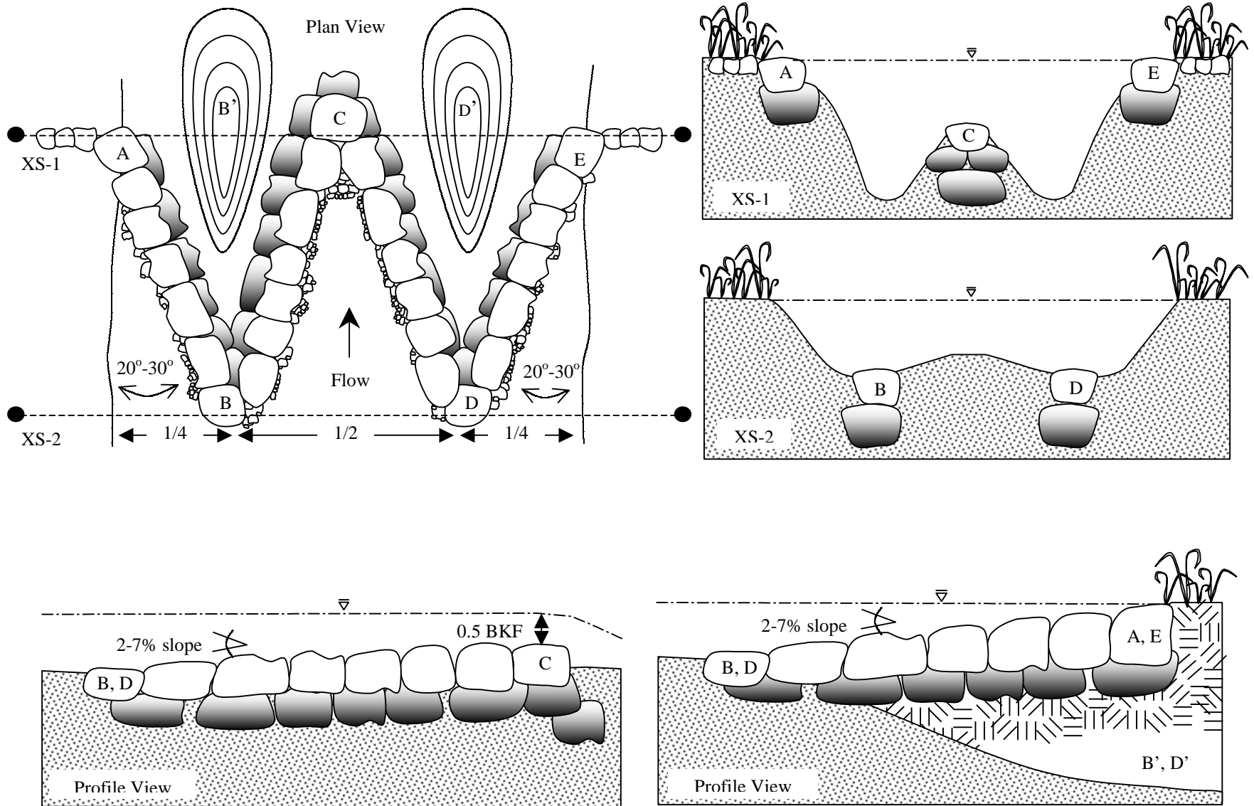
Figure 5. Plan, cross section, and profile views of the W-weir
