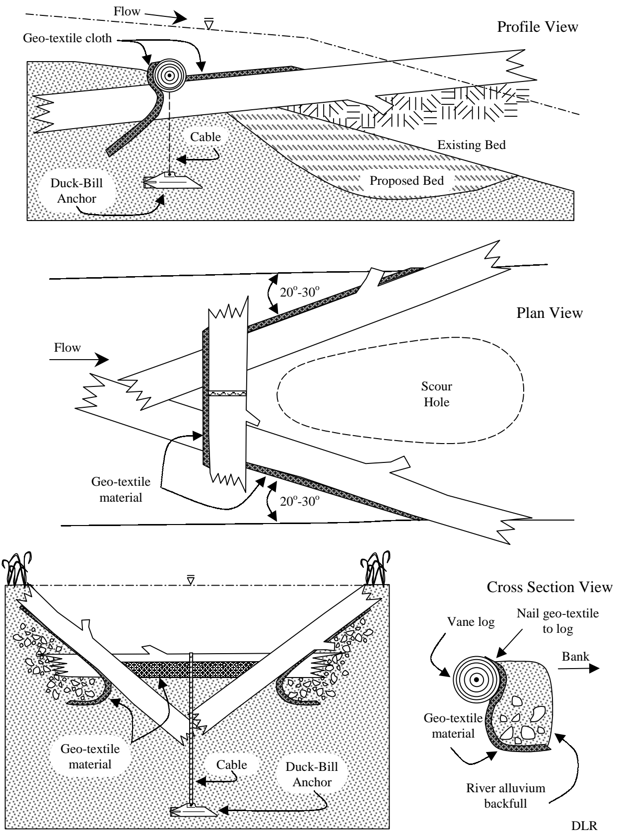
Figure 11. Cross-Vane using logs and a duck-bill anchor
