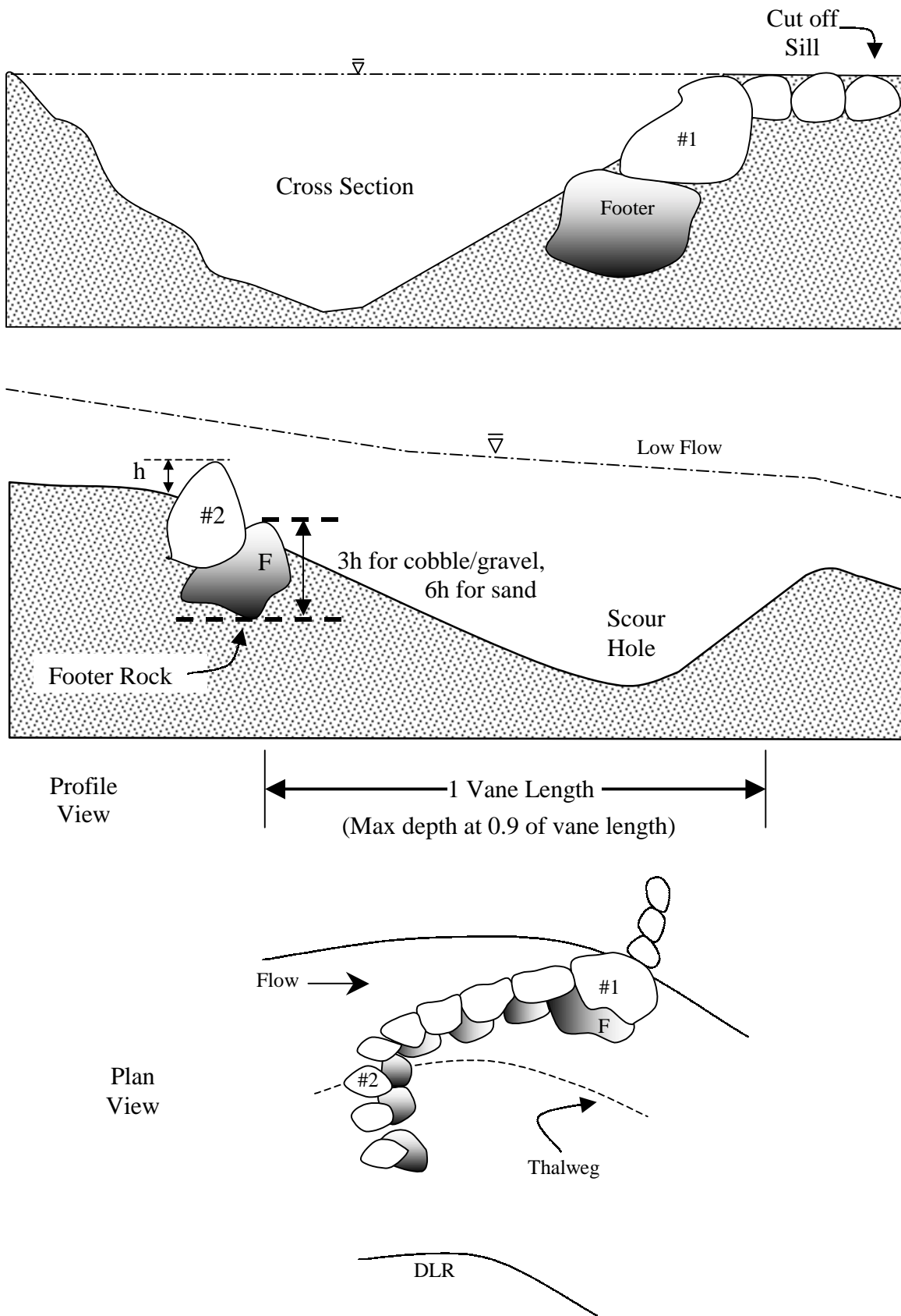
Figure 9. Locations/positions of rocks and footers in relation to channel shape and depths
