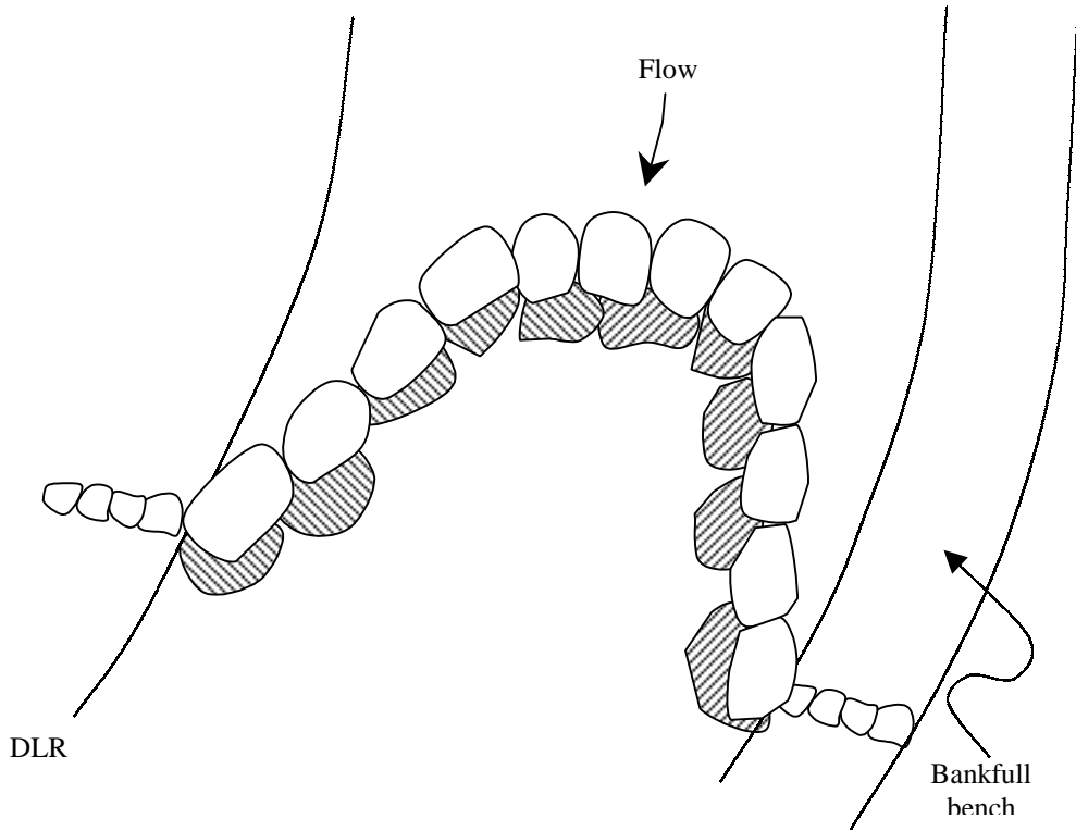
Figure 8. Example of a boulder Cross-Vane and constructed bankfull bench
