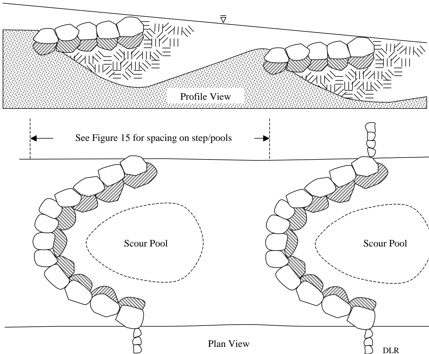
Figure 14. Use of Cross-Vane for step/pool restoration
