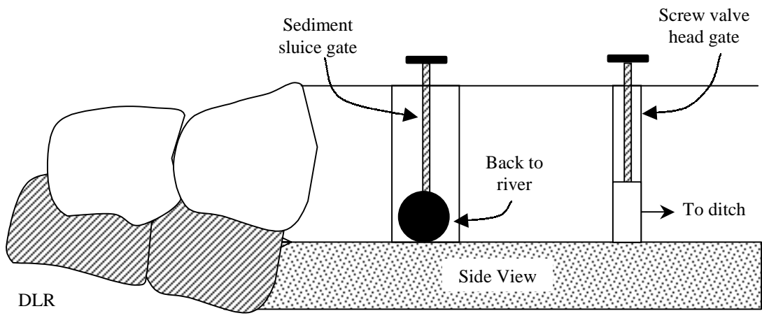
Figure 13. Example of a Cross-Vane/irrigation head gate-sediment sluice
