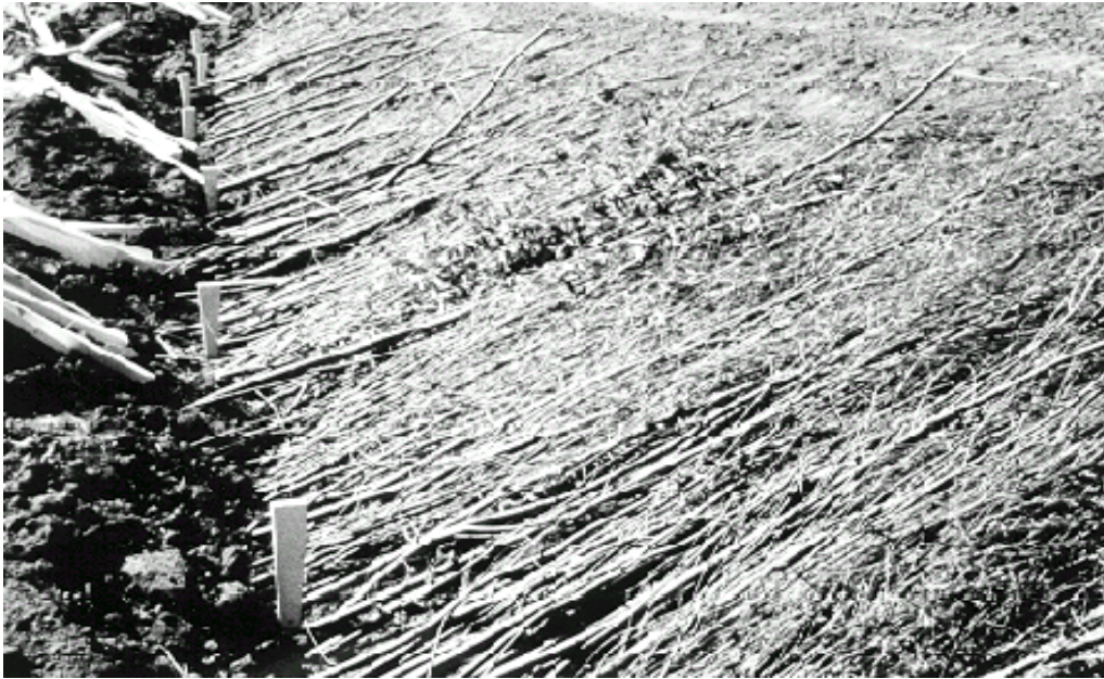
5.26a. Brush placed in a mattress before backfilling
