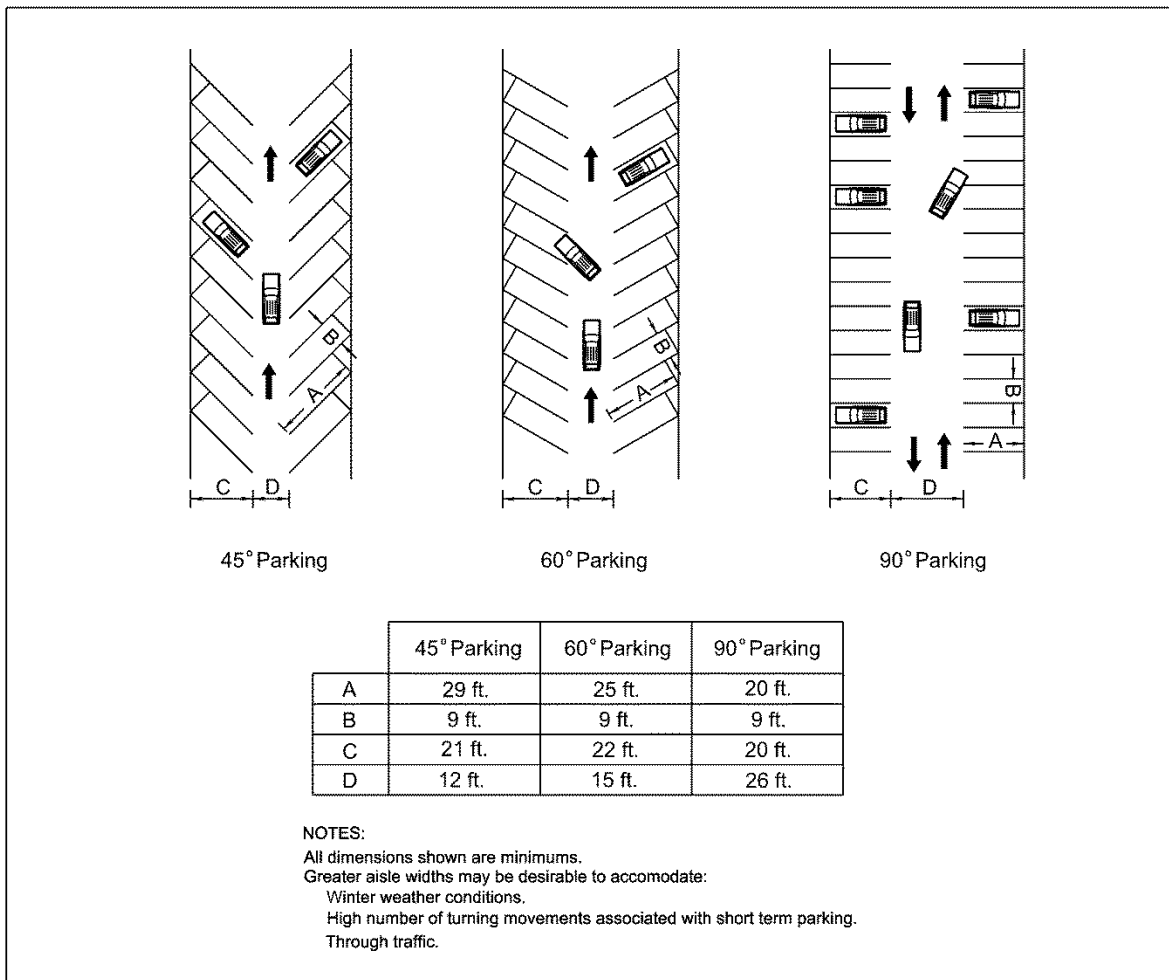
FIGURE C-1-14 PARKING SPACE DESIGN AND ARRANGEMENT FOR PARKING LOTS AND PARK & RIDE LOTS
