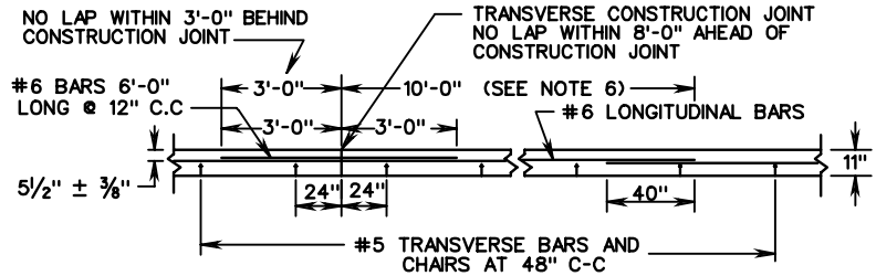
SECTION B-B DOUBLE LAP METHOD
