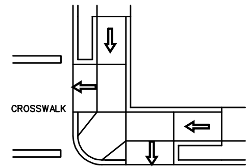
TYPICAL PLACEMENT AT INTERSECTION WITH BUFFER STRIP
