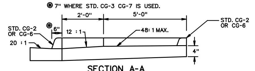
TYPICAL PLACEMENT AT INTERSECTION WITH BUFFER STRIP
