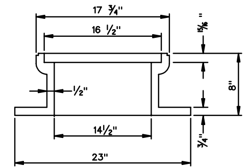
TYPE "D" VALVE BOX
