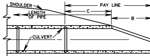
SLOPE DETAIL
