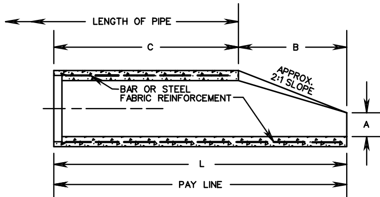
SECTION X-X
