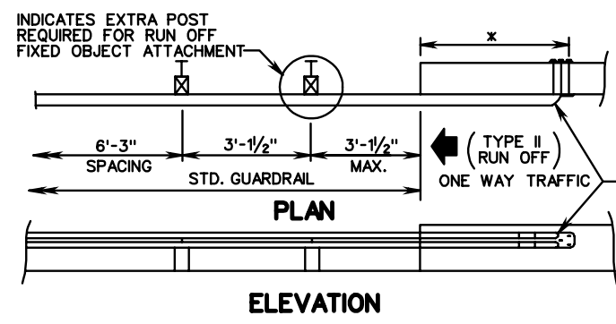
ITEM 8 DETAIL
