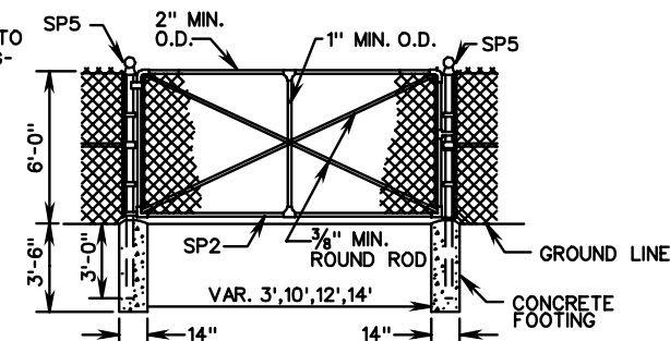
SINGLE SWING GATE
