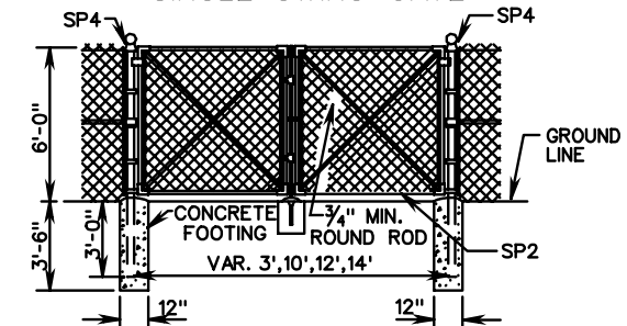
DOUBLE SWING GATE
