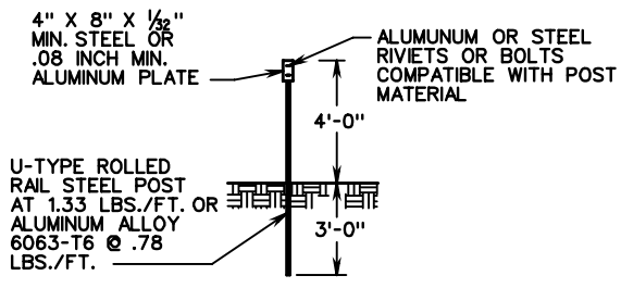
UNDERDRAIN OUTLET MARKER DETAIL
