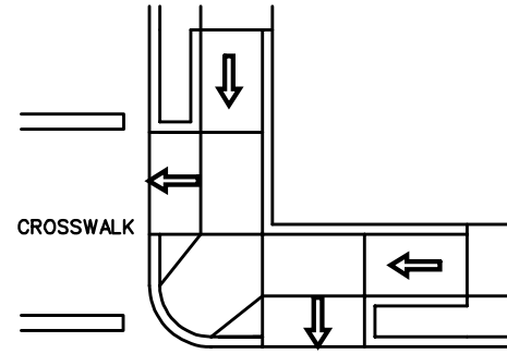
TYPICAL PLACEMENT AT INTERSECTION WITH BUFFER STRIP
