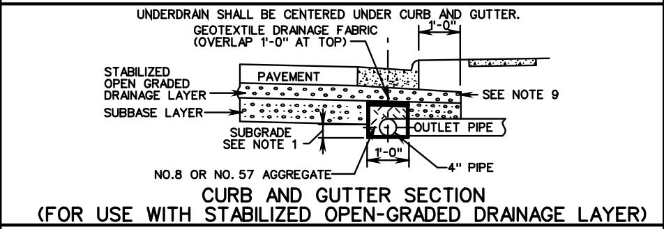
PAVED SHOULDER SECTION (FOR USE WITH STABILIZED OPEN-GRADED DRAINAGE LAYER)
