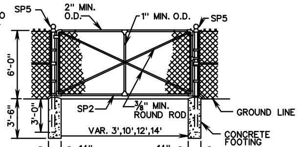
SINGLE SWING GATE
