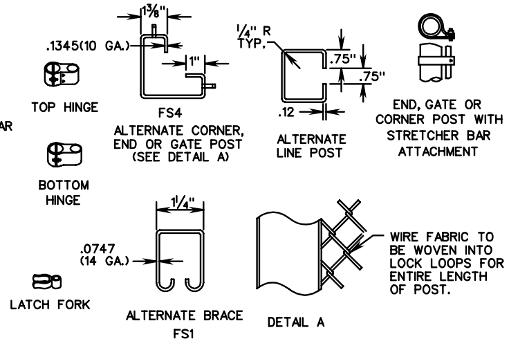
BOTTOM GATE CORNER & HINGE ATTACHMENT
