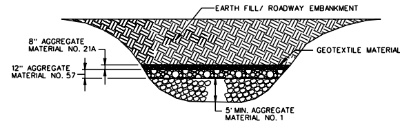
DETAIL NO. 3
