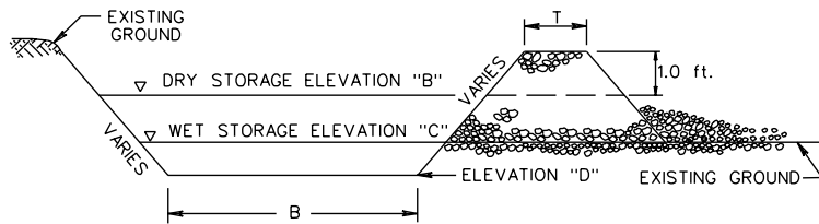
TYPICAL SECTION (A-A) THRU TEMPORARY SEDIMENT TRAP
