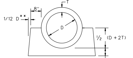
CONCRETE CRADLE
