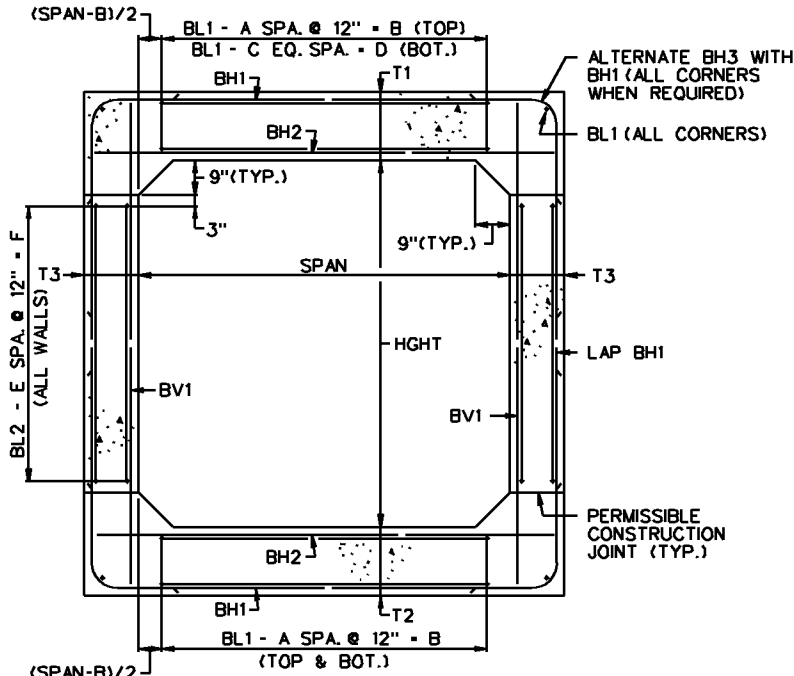
TYPICAL SECTION
