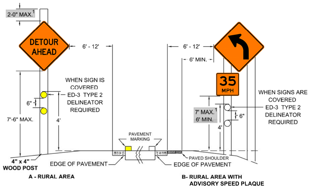
Figure 6F-1, Height and Lateral Location of Signs – Typical Post-Mounted Installations
