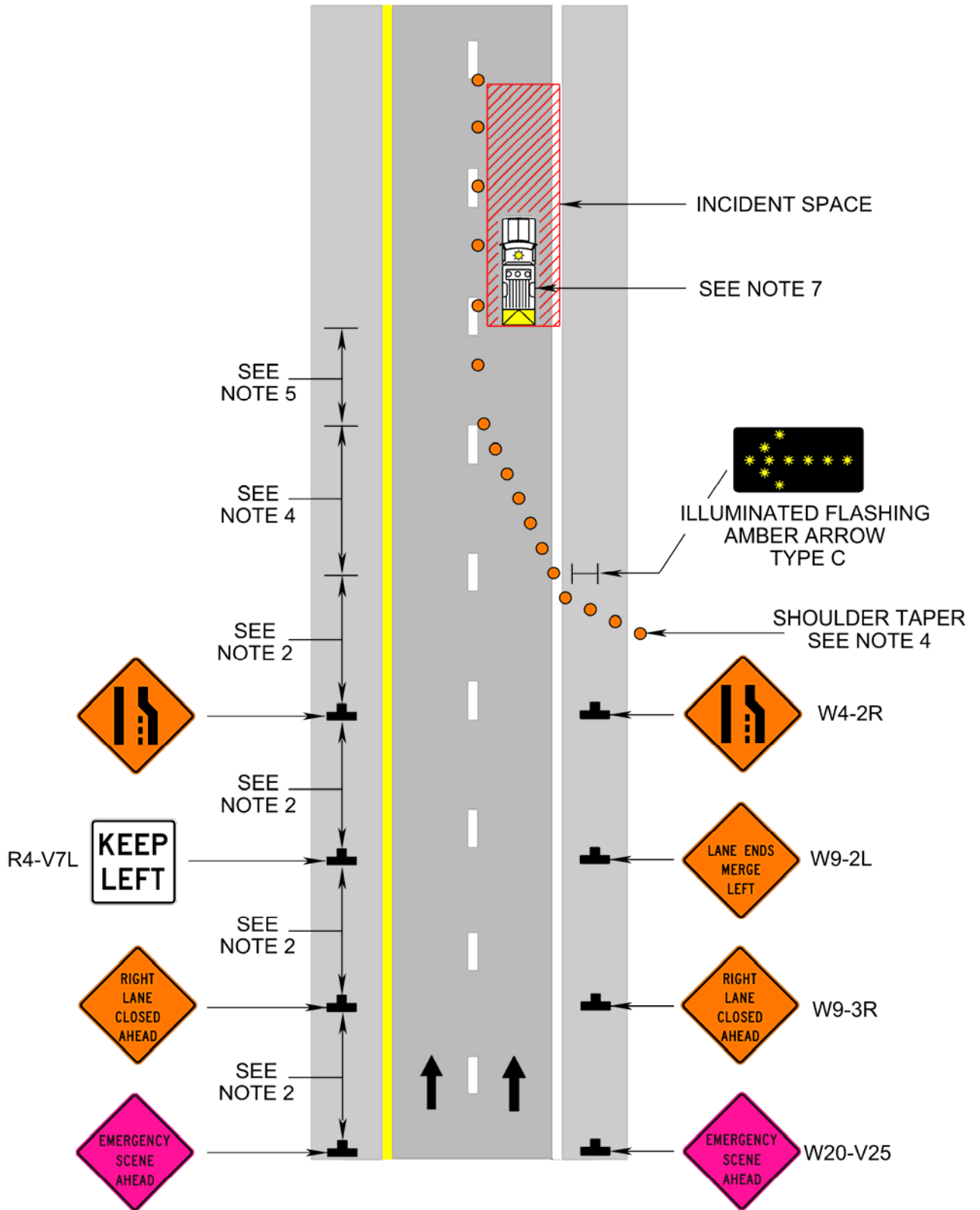
Incident in Outside Lane on Four-Lane Roadway (Figure TIMC-2.1)
