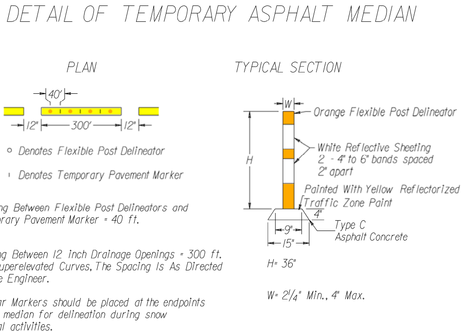
Figure 6, Temporary Asphalt Median Detail
