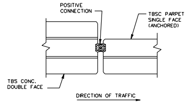
PLAN OF POSITIVE CONNECTION
