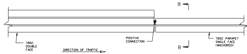
PLAN VIEW METHOD A
