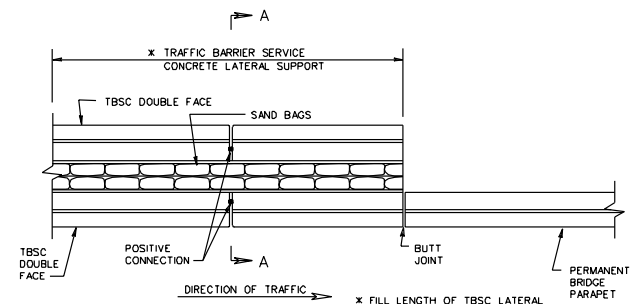
PLAN VIEW METHOD B
