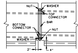
ELEVATION OF POSITIVE CONNECTION
