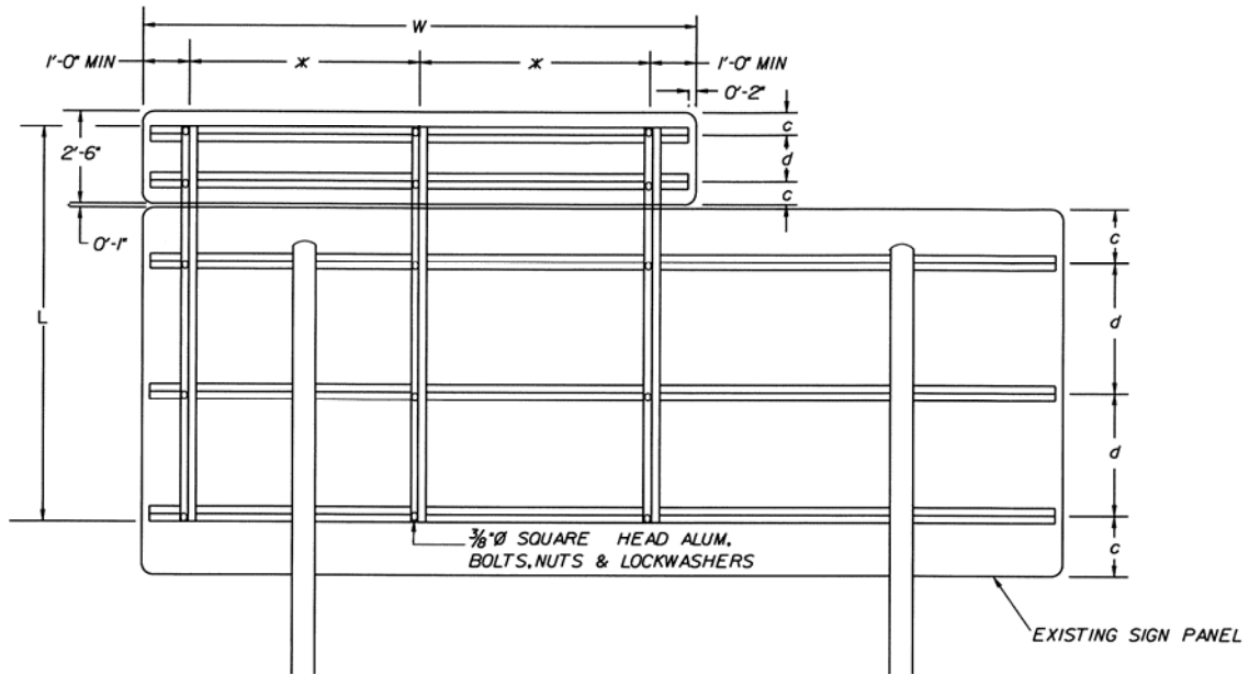
Appendix IIA-10: TYPICAL DETAILS FOR MOUNTING EXIT NUMBER SIGN PANELS (Enlarged View)
