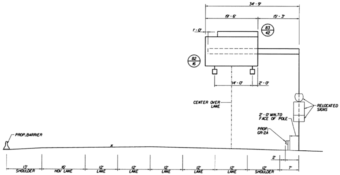
OVERHEAD STRUCTURE LOCATION 30 STA. 1012-75 W.B. MAINLINE CONST.
