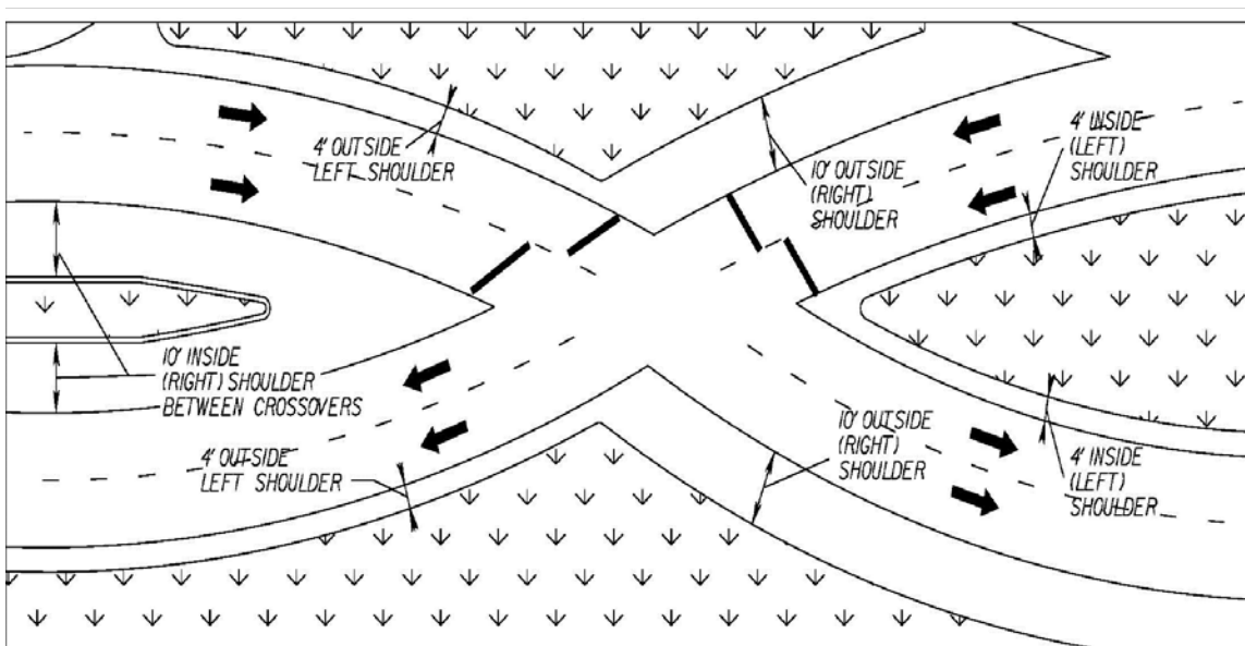
FIGURE A-3-6 SHOULDER DESIGN FOR DDI
