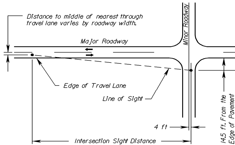
Left Sight Distance Triangle
