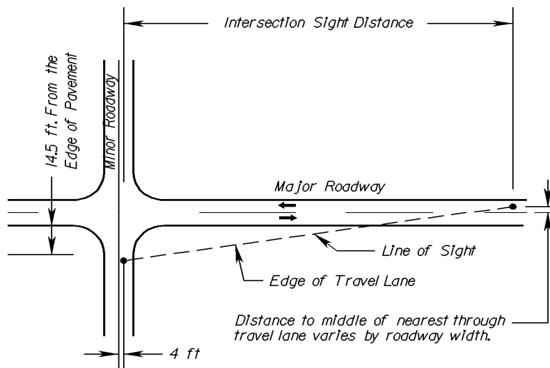
Right Sight Distance Triangle
