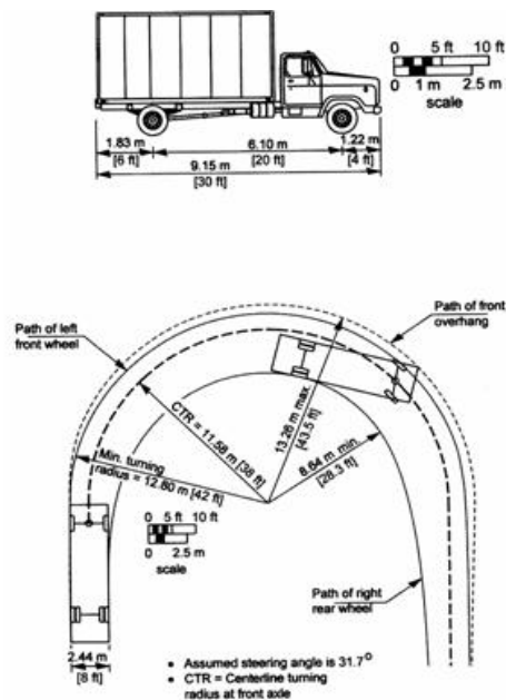
FIGURE 1 – "EXHIBIT 2-4" SCANNED FROM "A POLICY ON GEOMETRIC DESIGN OF HIGHWAYS AND STREETS," AASHTO, 2004
