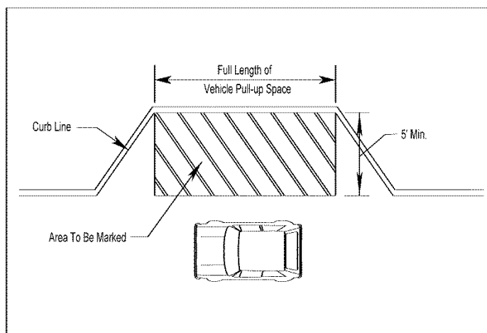
FIGURE A(1)-2-5 ACCESS AISLE (R310.3)
