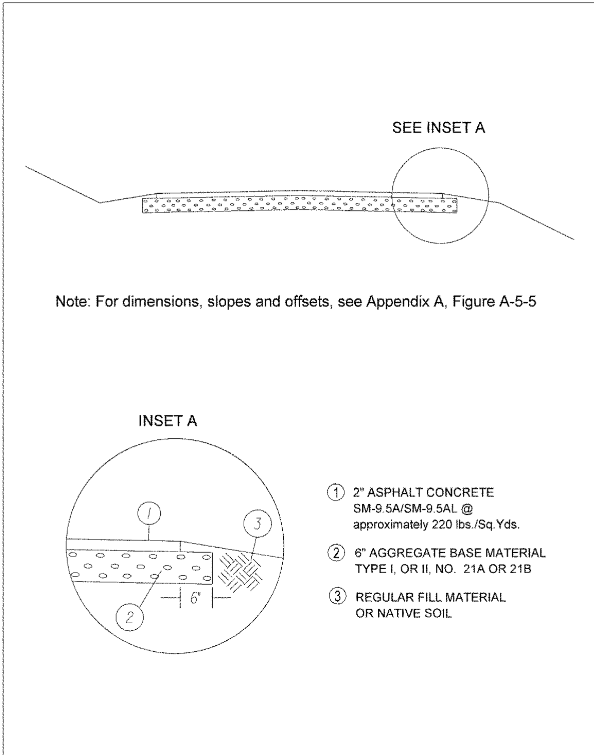
FIGURE A(1)-1-10 SHARED USE PATH PAVEMENT STRUCTURE
