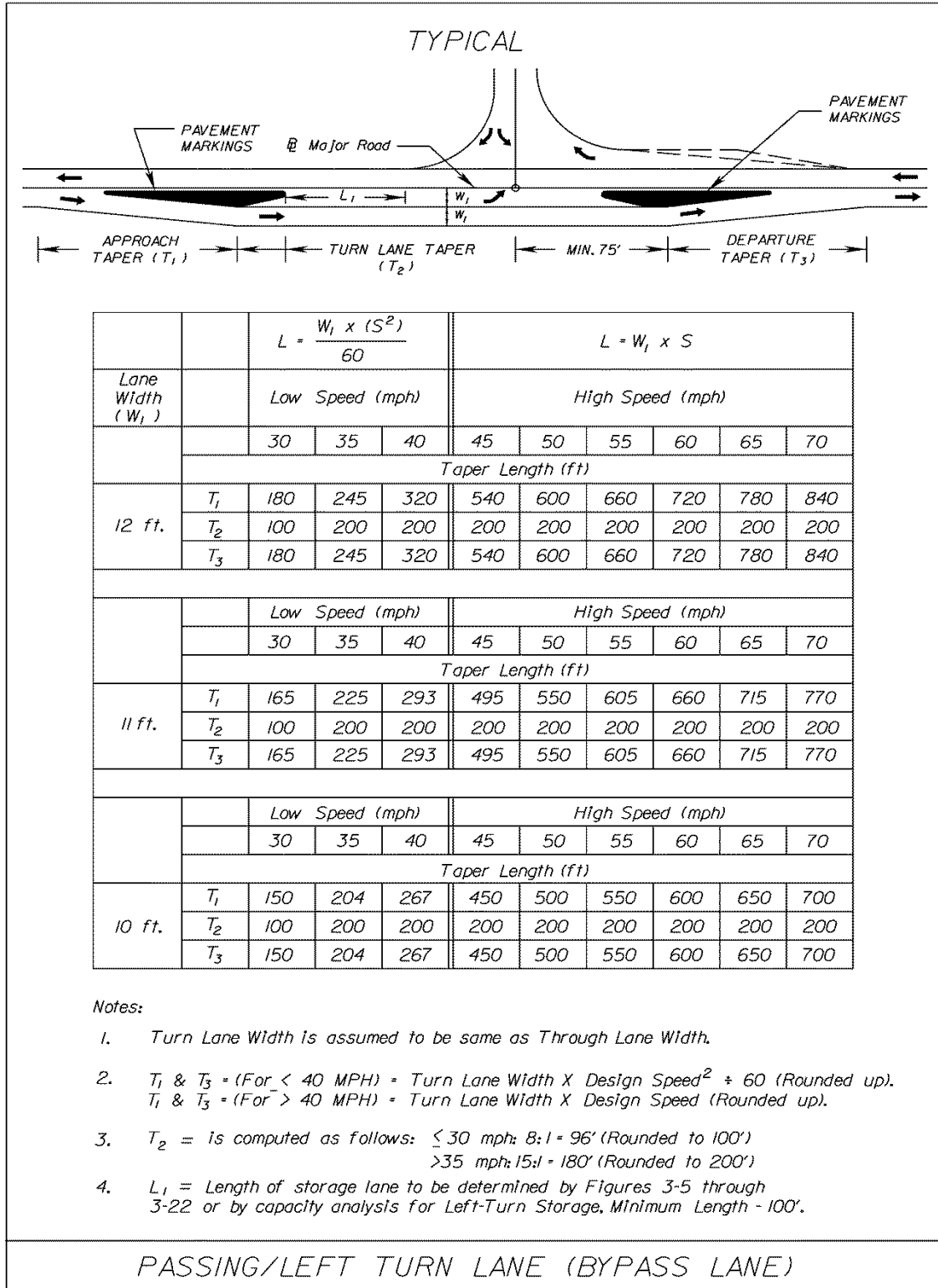
FIGURE 3-4 PASSING/LEFT TURN LANE
