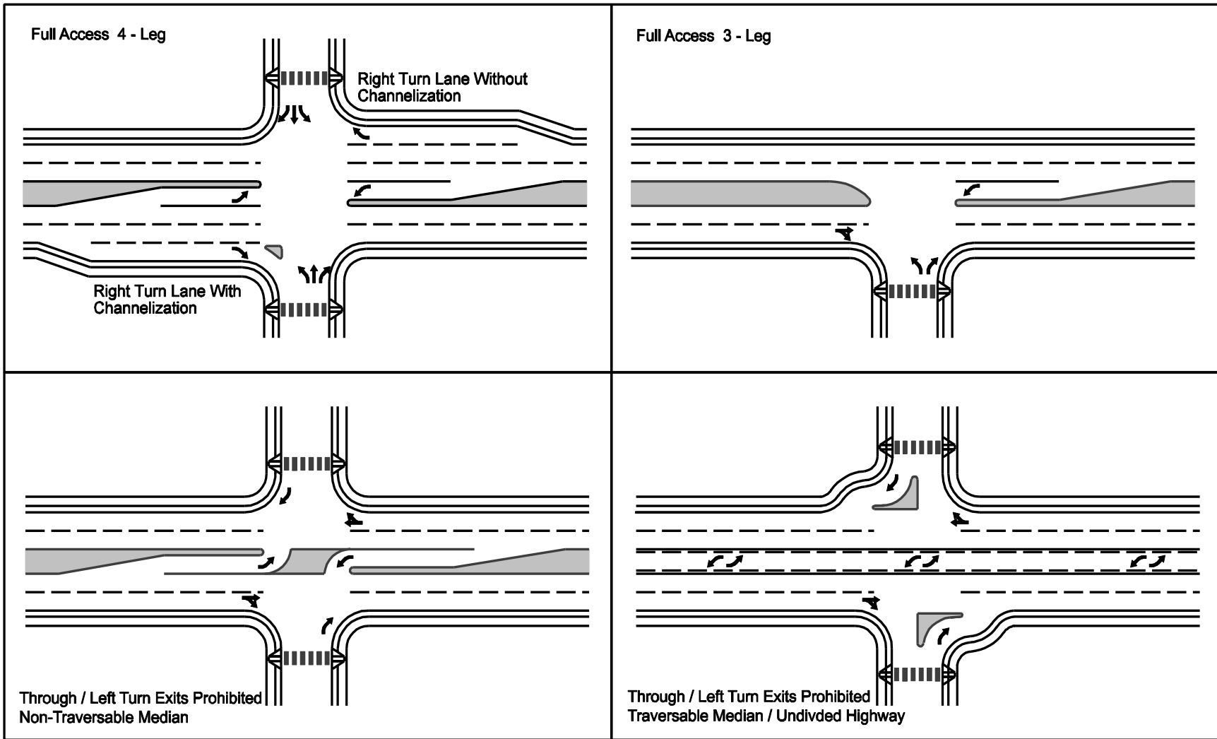
FIGURE 2-3 TYPES OF ACCESS CHANNELIZATION
