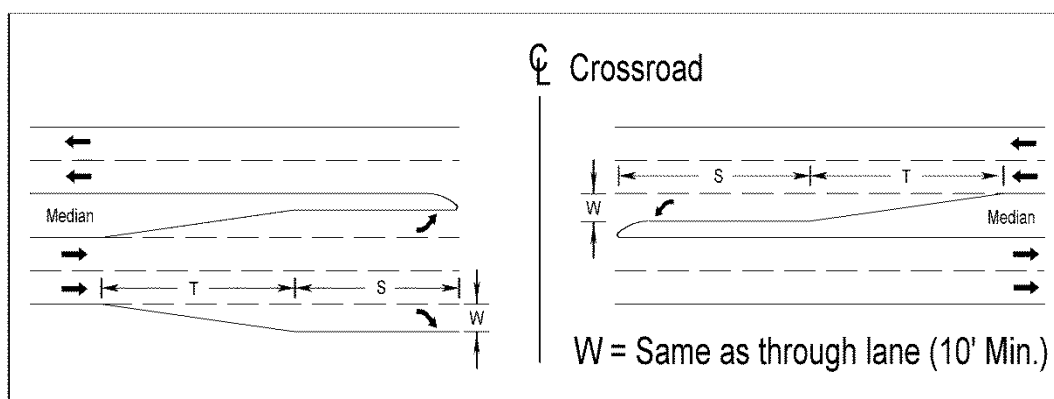
FIGURE 3-2 LEFT AND RIGHT TURN STORAGE AND TAPER LENGTHS
