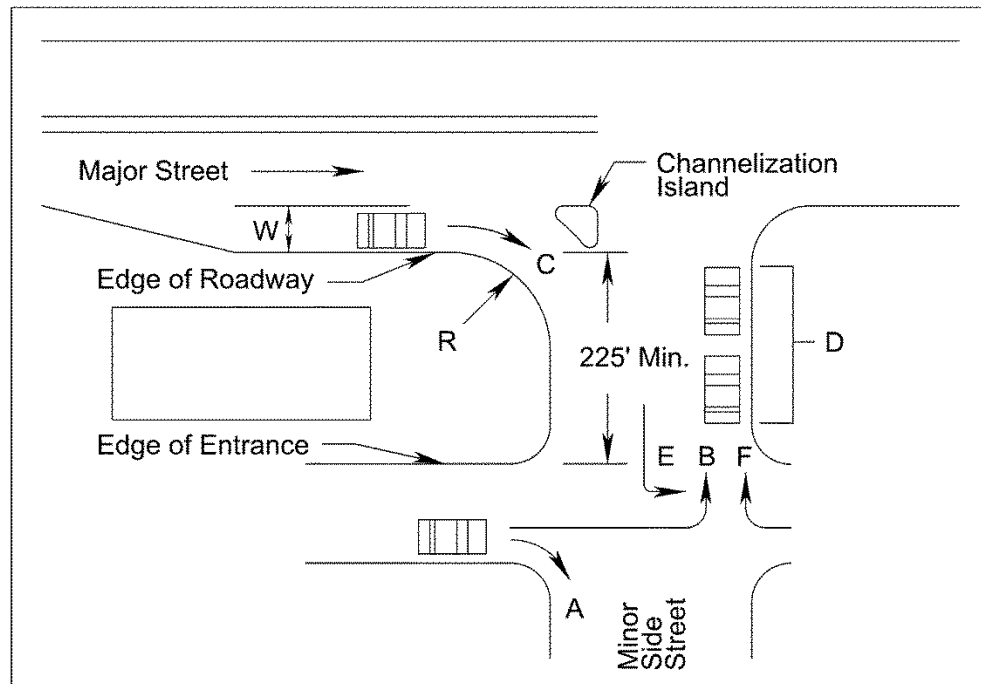
FIGURE 4-5 CORNER CLEARANCE
