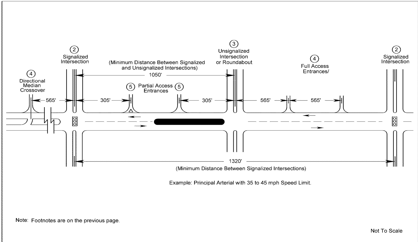
FIGURE 2-8.1 ILLUSTRATION OF THE RELATIONSHIP BETWEEN SPACING STANDARDS*
