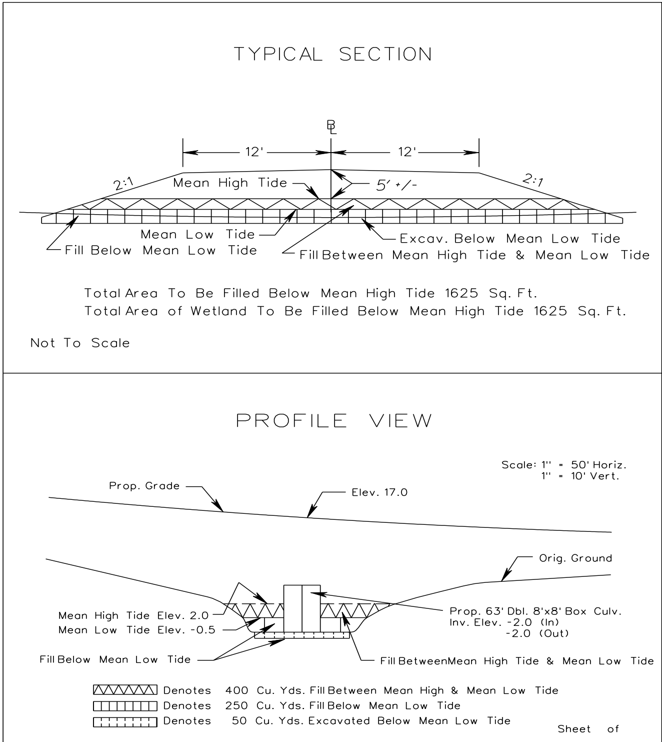
FIGURE C-4-9 CULVERT (TIDAL) –TYPICAL SECTION & PROFILE VIEW
