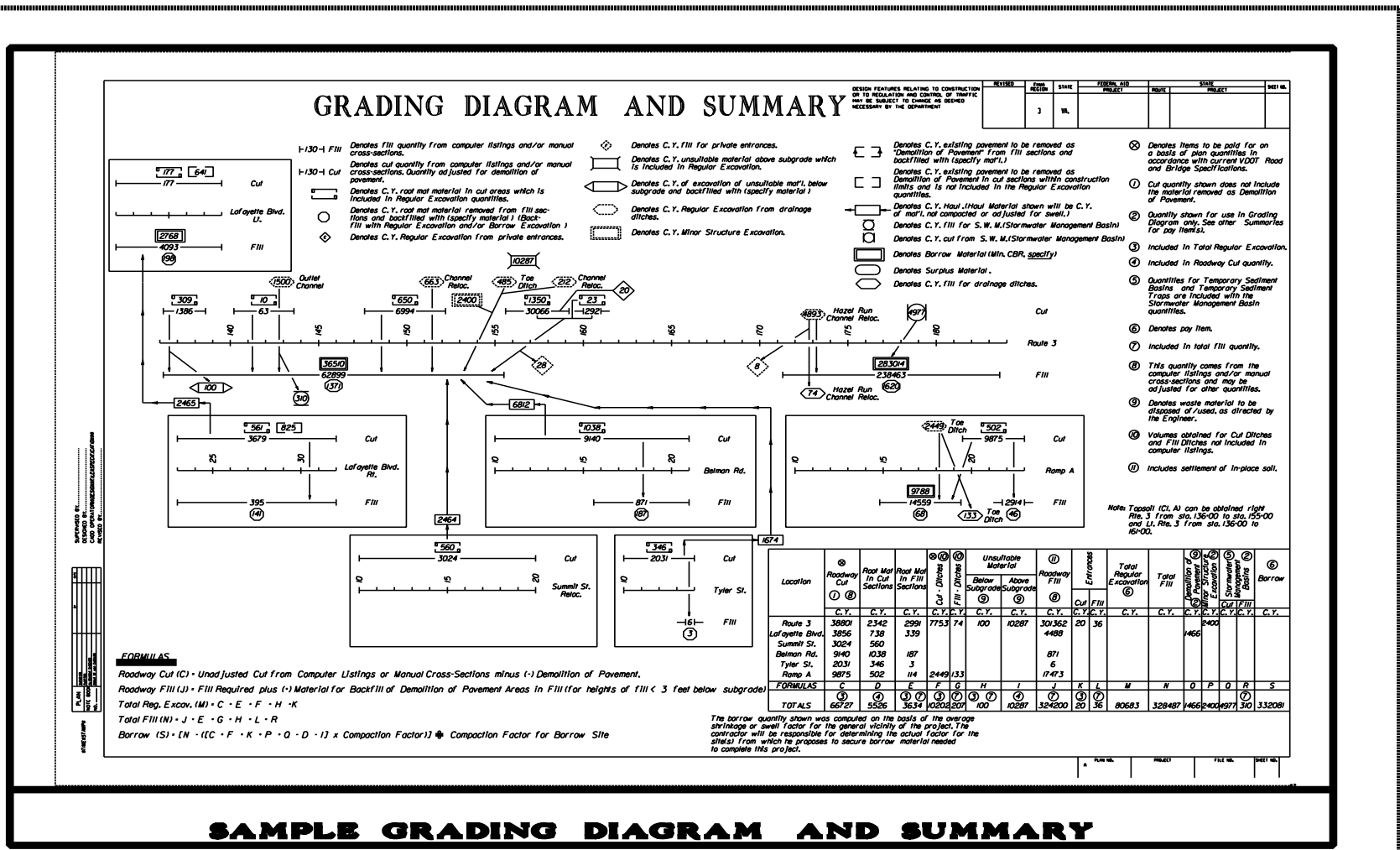
FIGURE 2G-3 SAMPLE GRADING DIAGRAM AND SUMMARY SHEET*
