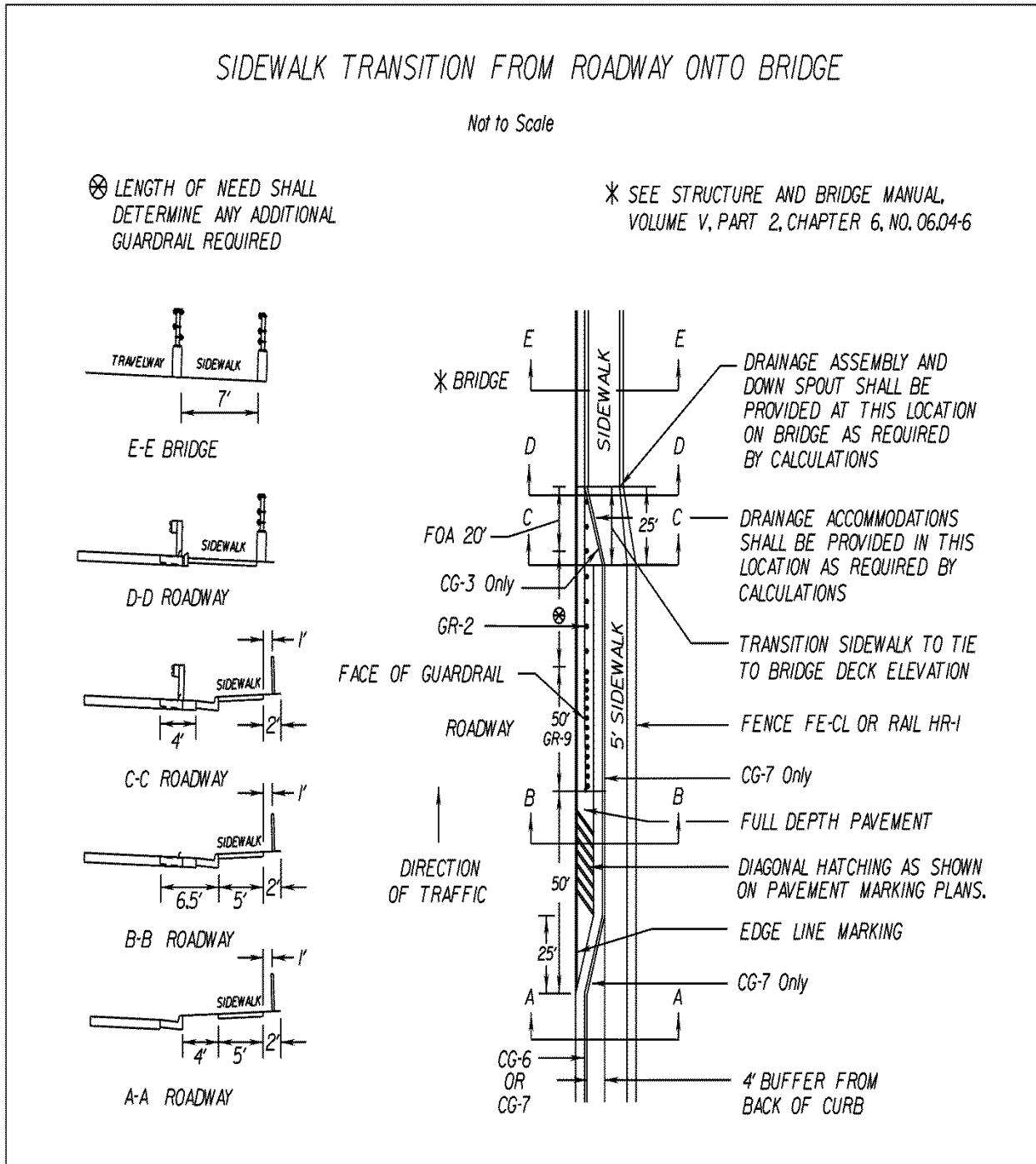
FIGURE A-5-22 SIDEWALK TRANSITION FROM ROADWAY ONTO BRIDGE FOR DESIGN SPEEDS >45 MPH*
