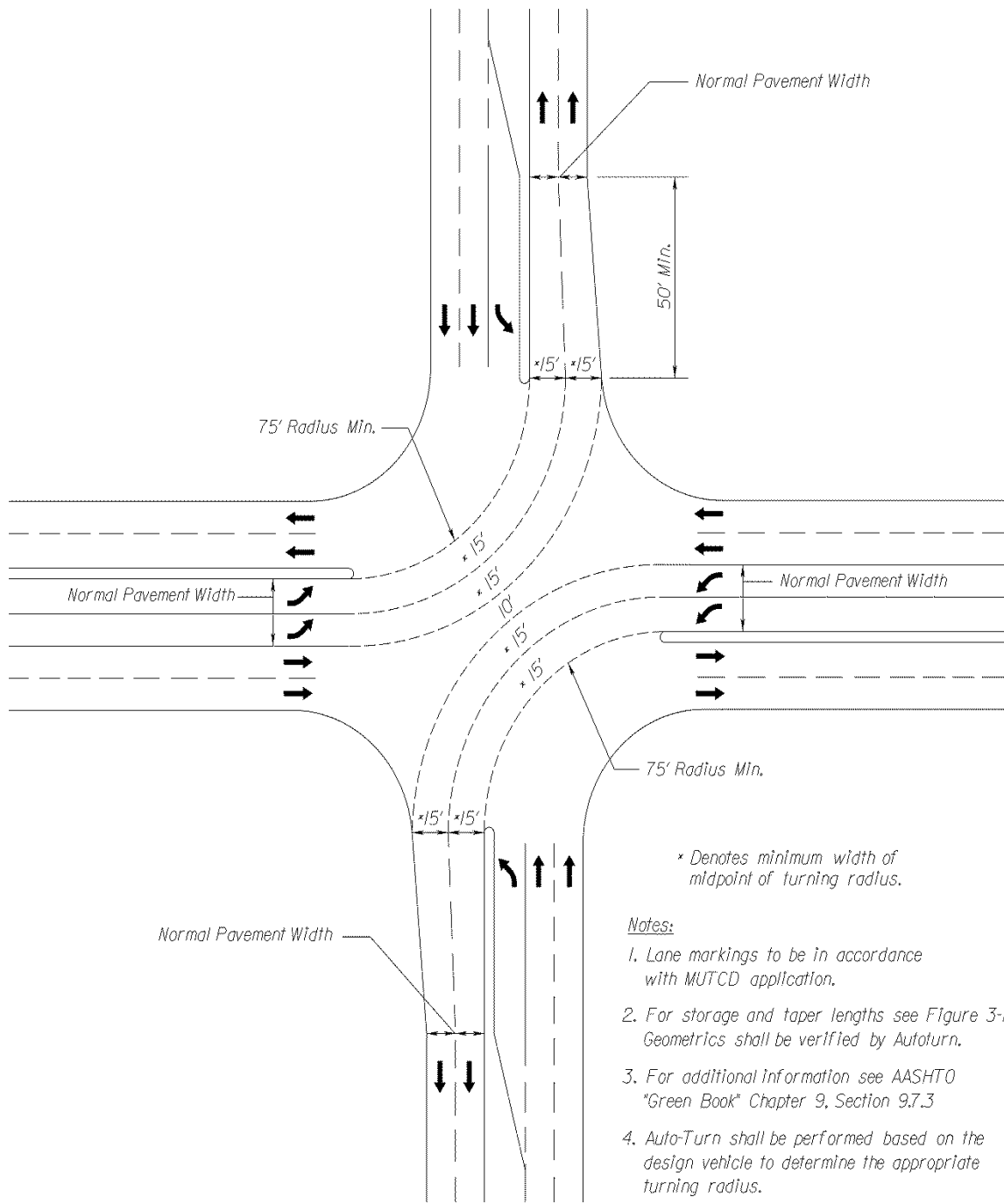
FIGURE 3-23 DOUBLE LEFT-TURN LANES*
