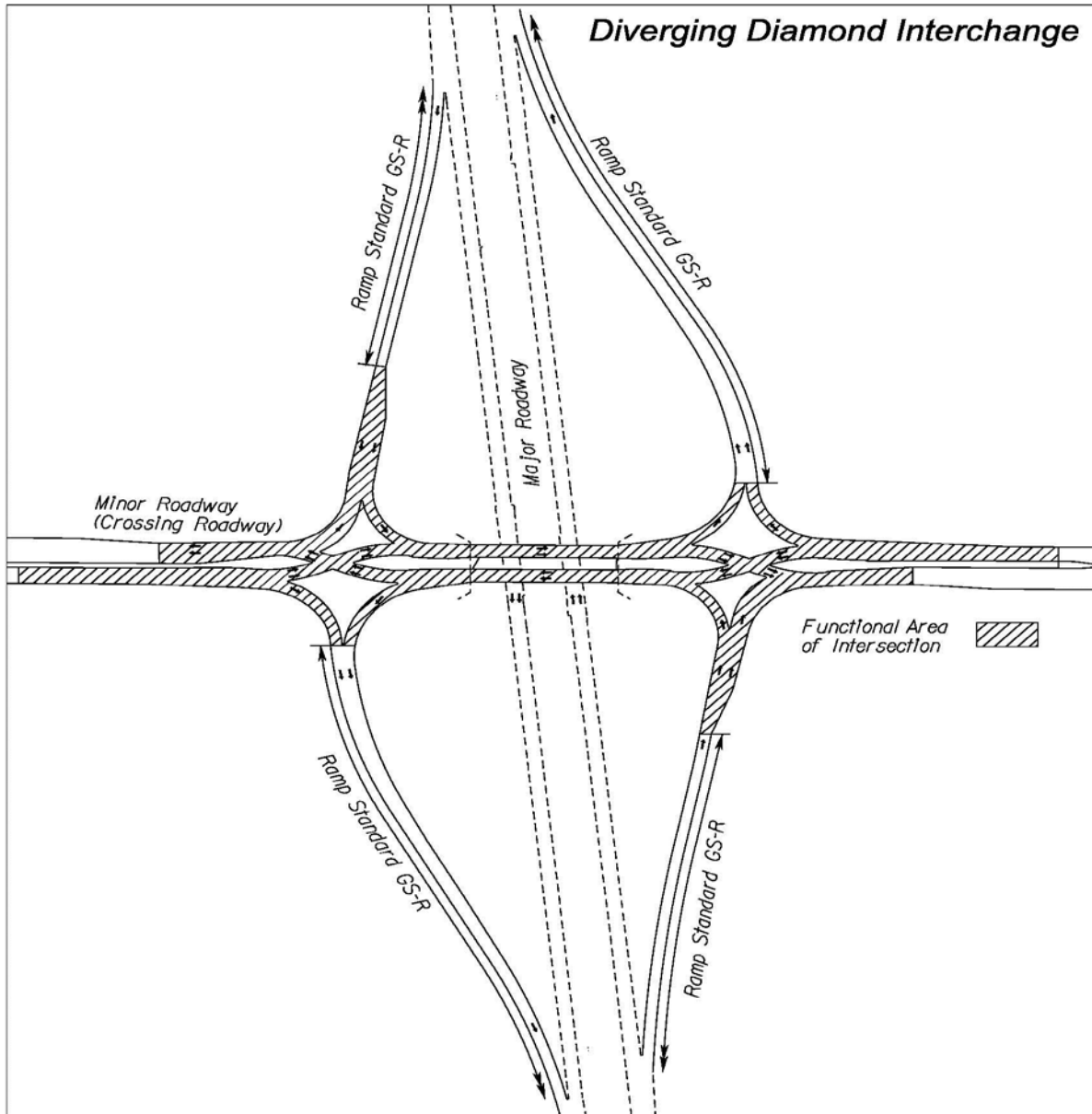
FIGURE 2-16 DIVERGING DIAMOND LAYOUT
