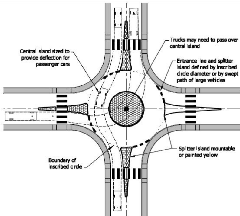
FIGURE 2-15 MINI-ROUNDBOULT DESIGN ELEMENTS*
