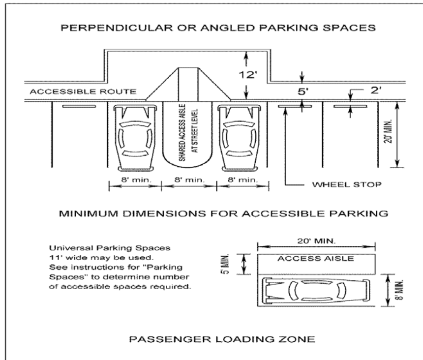
FIGURE C-1-3 ACCESSIBLE PARKING AND LOADING ZONES
