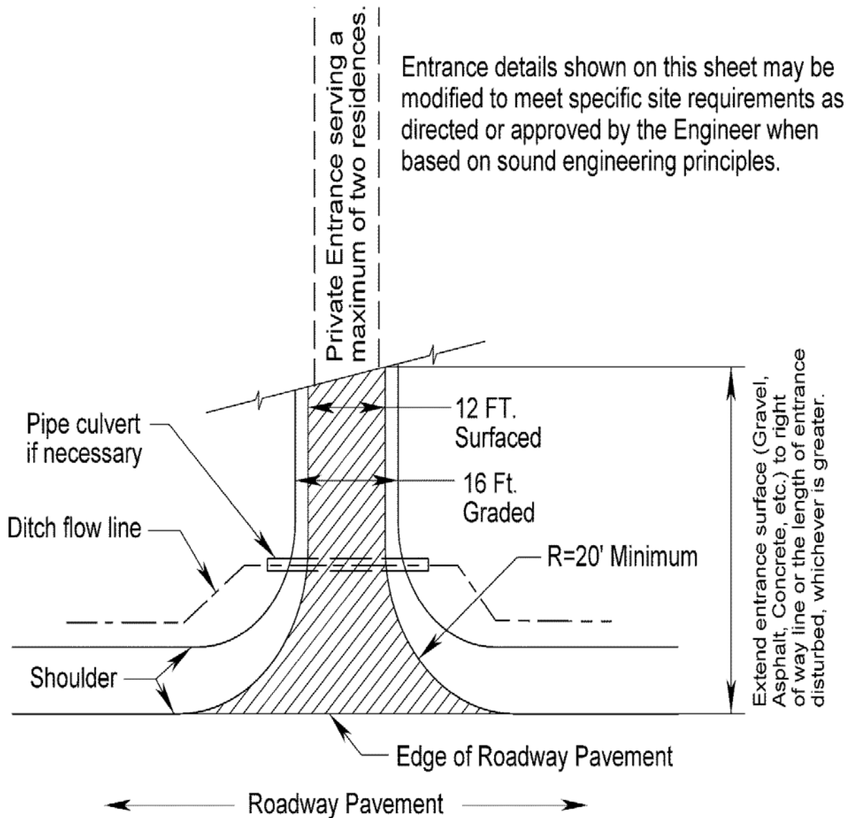
FIGURE 4-1 PRIVATE ENTRANCE AND LOW VOLUME COMMERCIAL ENTRANCE DETAIL*
