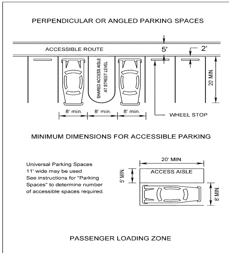
FIGURE C-1-3 ACCESSIBLE PARKING AND LOADING ZONES*
