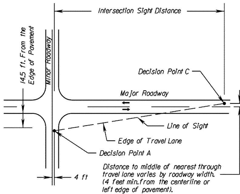
Right Sight Distance Triangle
