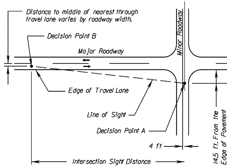
Left Sight Distance Triangle
