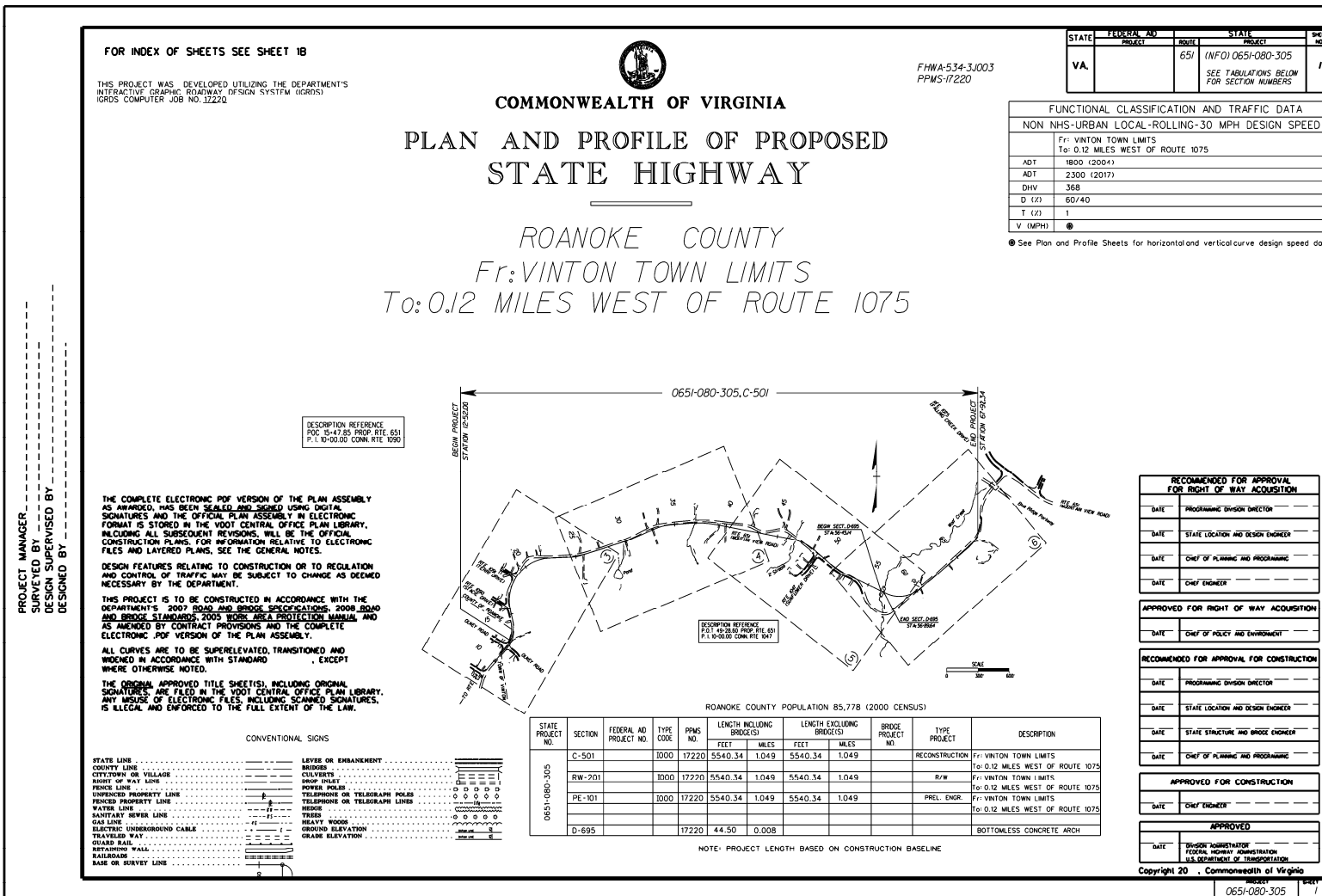
FIGURE 2E-11 SAMPLE TITLE SHEET (URBAN DESIGN)*
