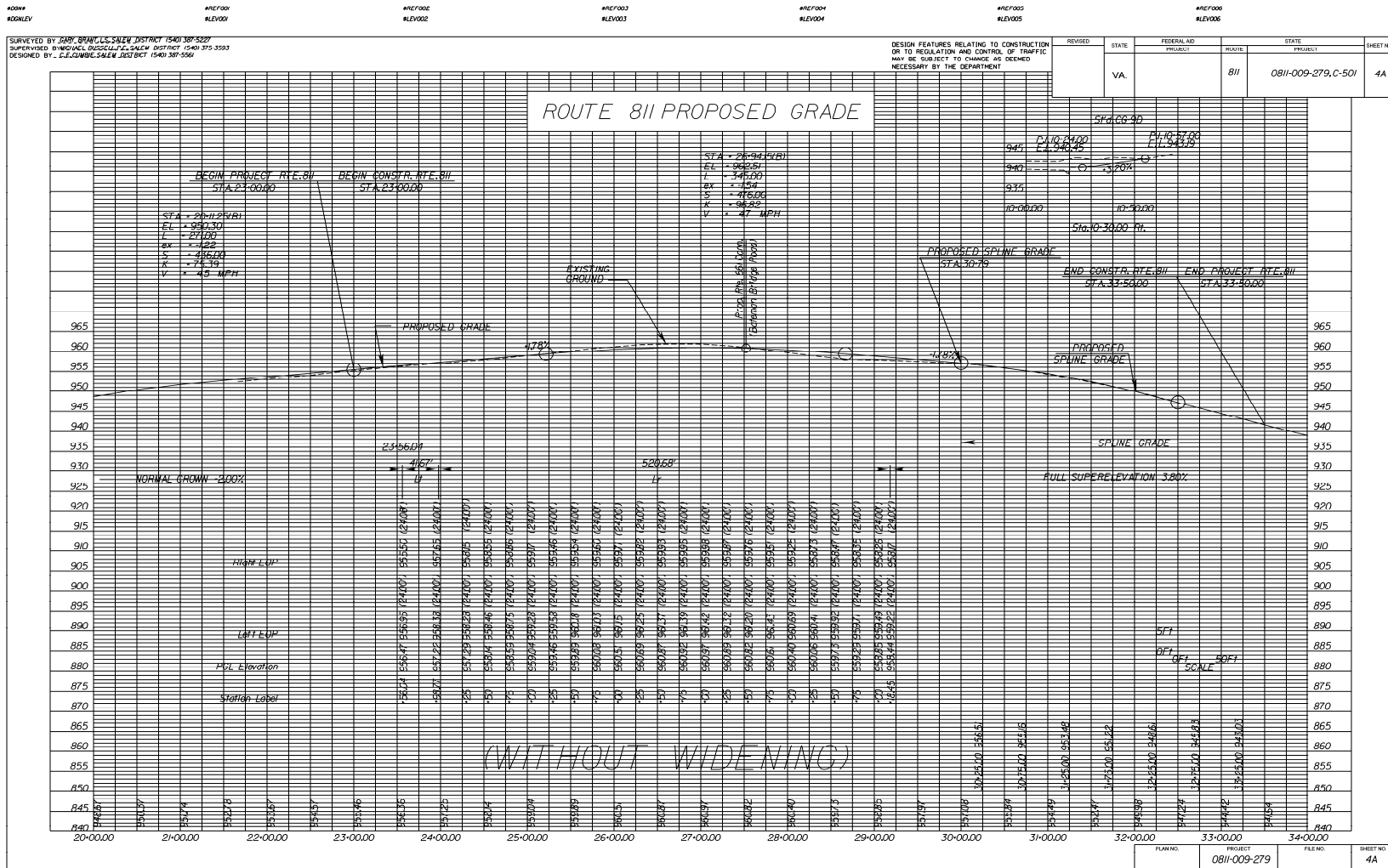
FIGURE 2D-3 SAMPLE PROFILE SHEET*
