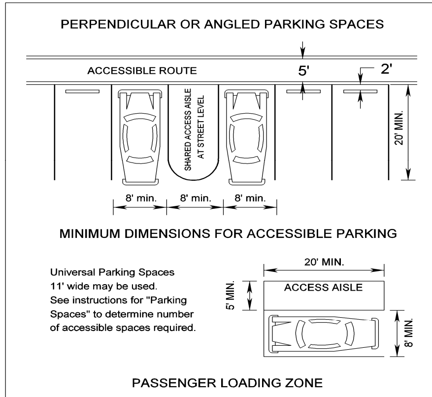
FIGURE C-1-3 ACCESSIBLE PARKING AND LOADING ZONES
