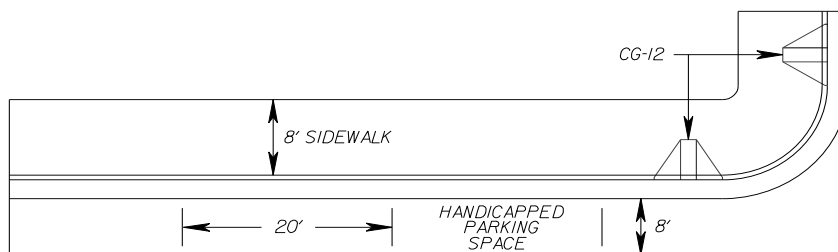
FIGURE C-1-2 DESIGNS FOR PARALLEL PARKING SPACES EXCEPTION
