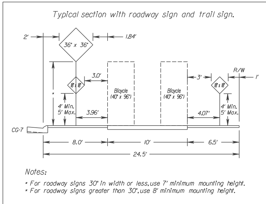
FIGURE A-5-4 SHARED USED PATHS
