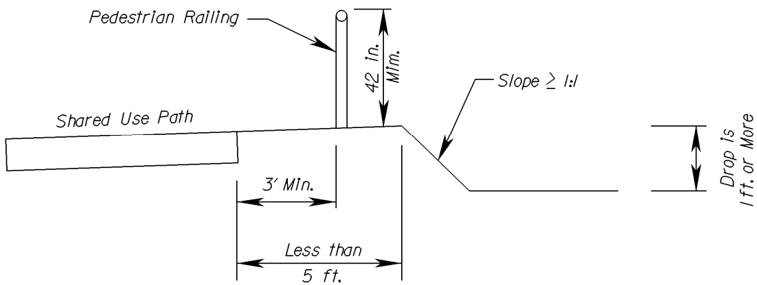
FIGURE A-5-6 PHYSICAL BARRIER FOR SHARED-USE PATH
