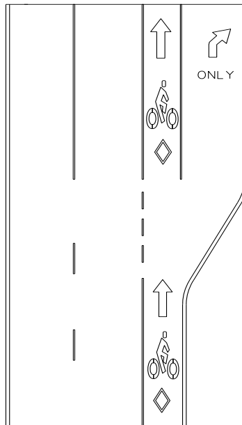
FIGURE A-5-3 RIGHT TURN ONLY LANE
