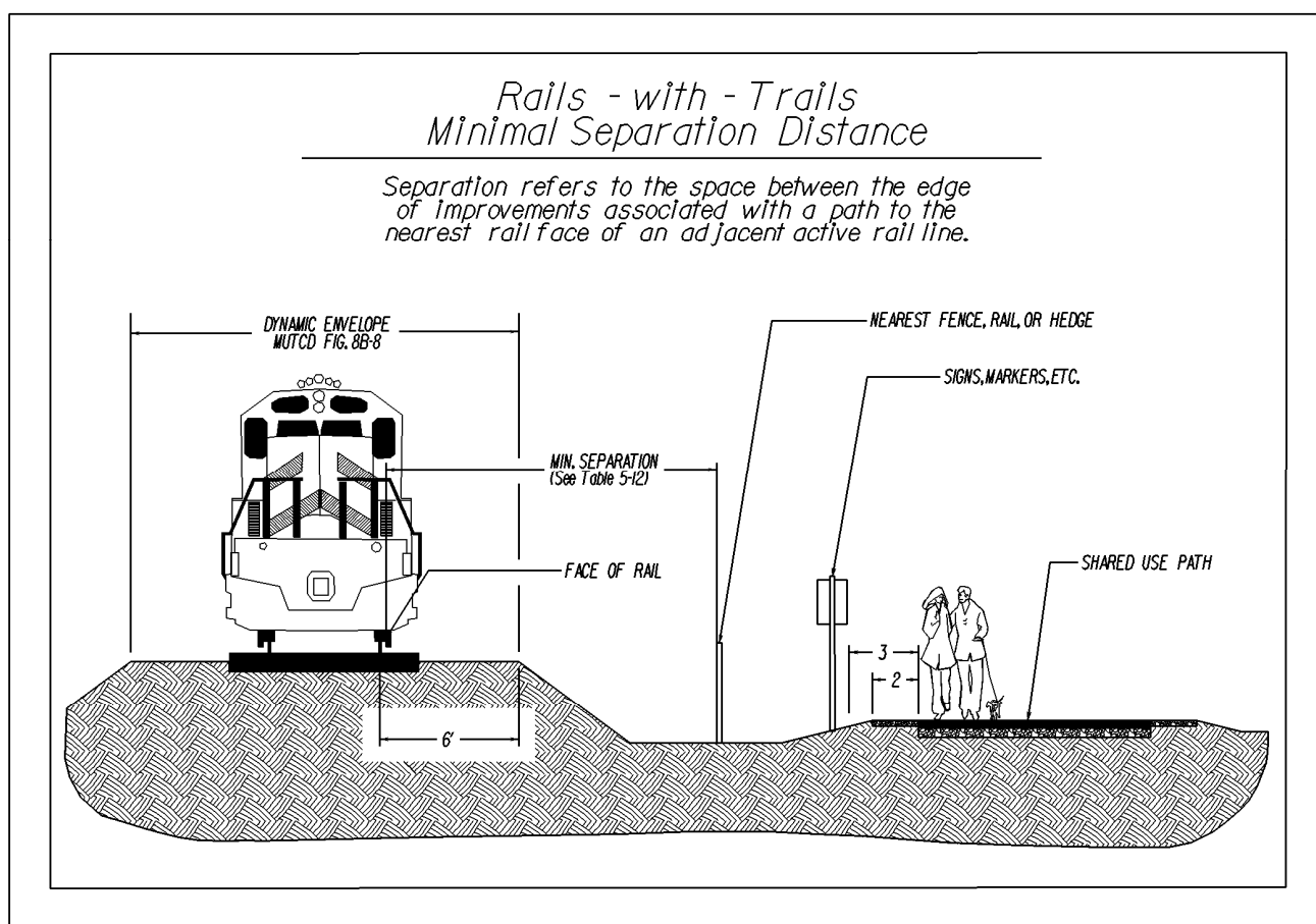
FIGURE A- 5-10 SEPARATION BETWEEN ACTIVE RAIL LINES AND PATHS (RWT)
