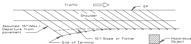
FIGURE A-3-2 SUGGESTED SLOPES FOR APPROACH BARRIERS
