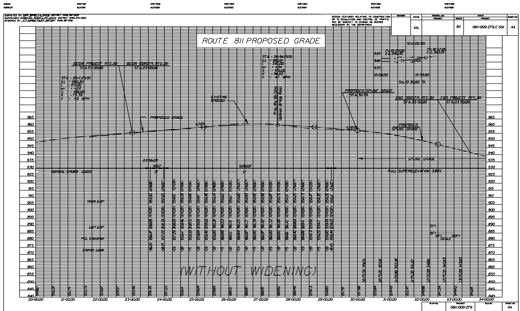
FIGURE 2D-4 SAMPLE PROFILE SHEET*
