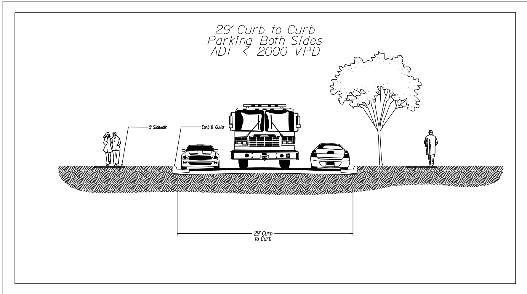
FIGURE 1.4 – 29' CURB TO CURB PARKING ON BOTH SIDES*
