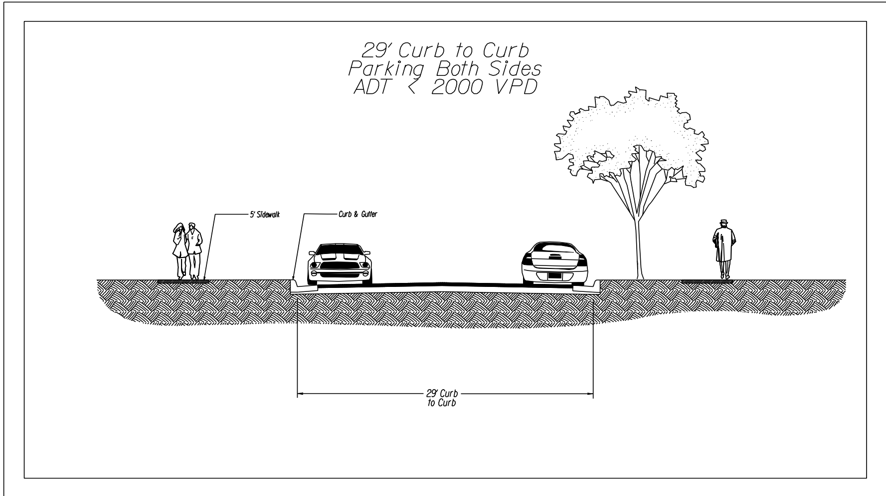
FIGURE 1.2 – 29' CURB TO CURB PARKING ON BOTH SIDES*
