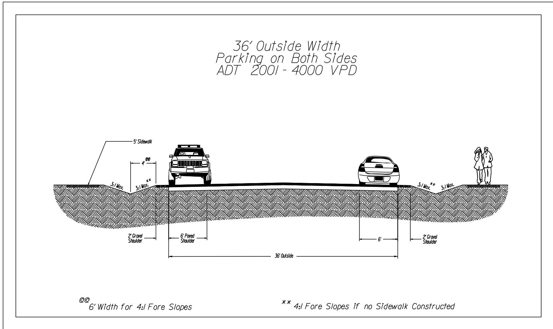
FIGURE 1.7 – 36' OUTSIDE WIDTH PARKING ON BOTH SIDES*
