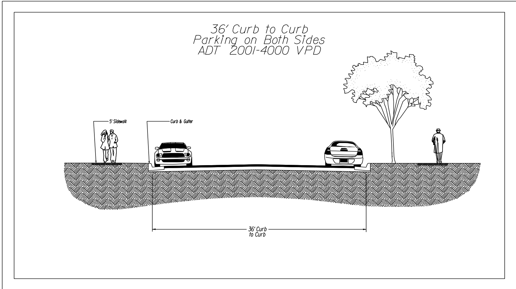
FIGURE 1.3 – 36' CURB TO CURB PARKING ON BOTH SIDES*
