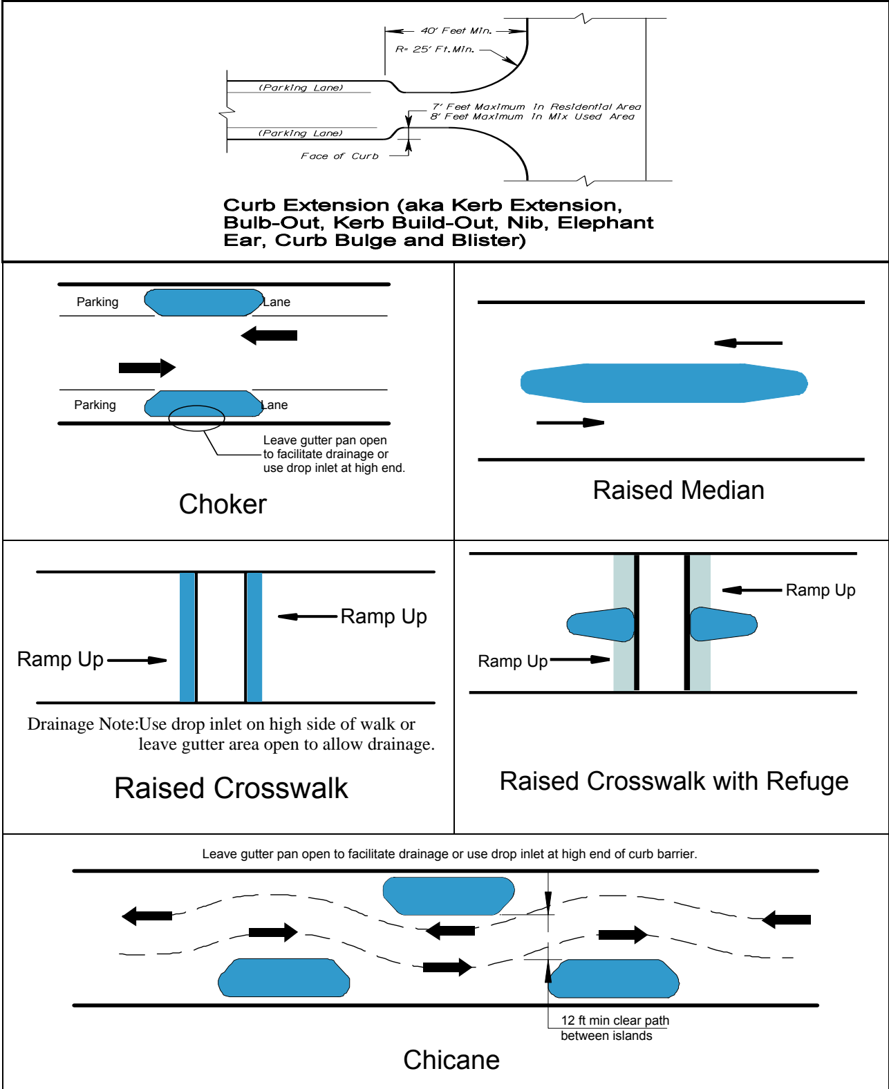
FIGURE 12 – TRAFFIC CALMING DETAILS*
