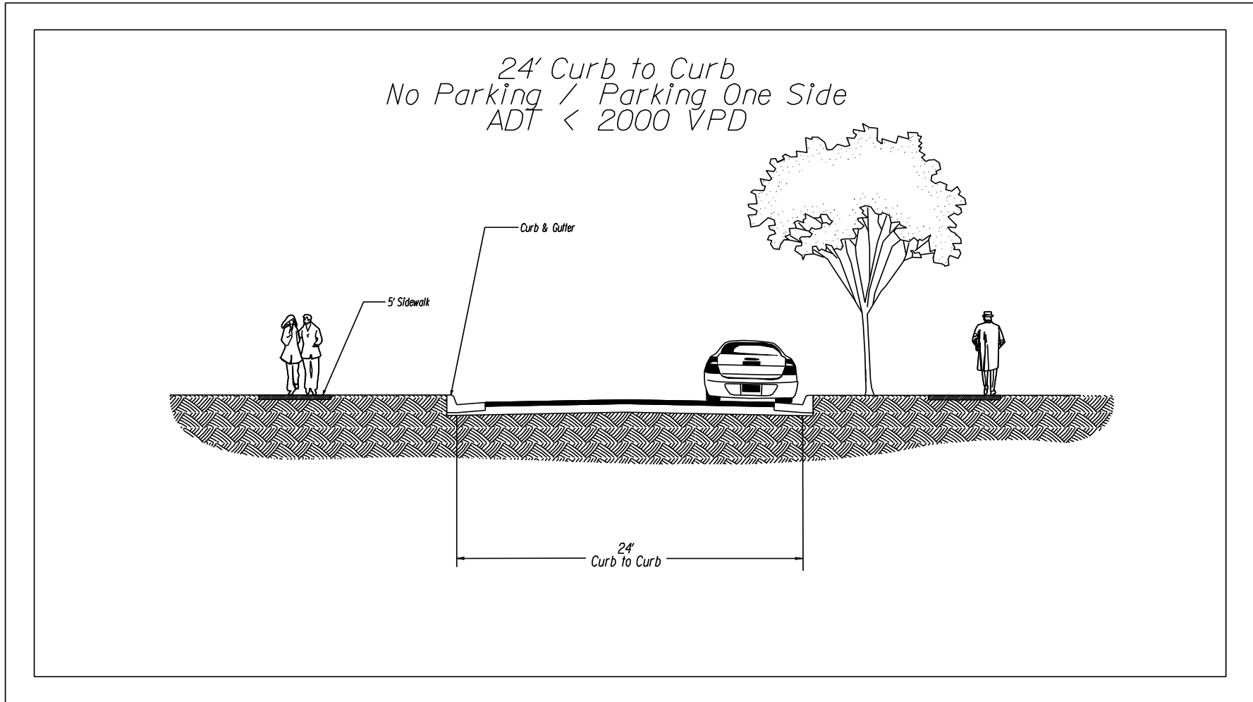
FIGURE 1.1 – 24' CURB TO CURB NO PARKING / PARKING ON ONE SIDE*
