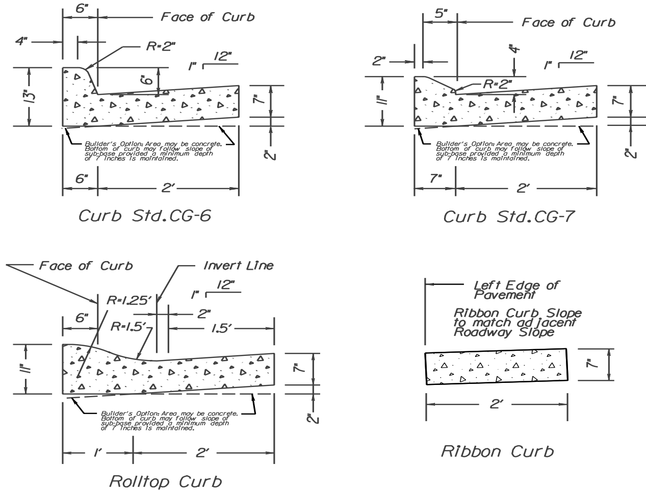
FIGURE 5 – CURB AND GUTTER DETAILS*
