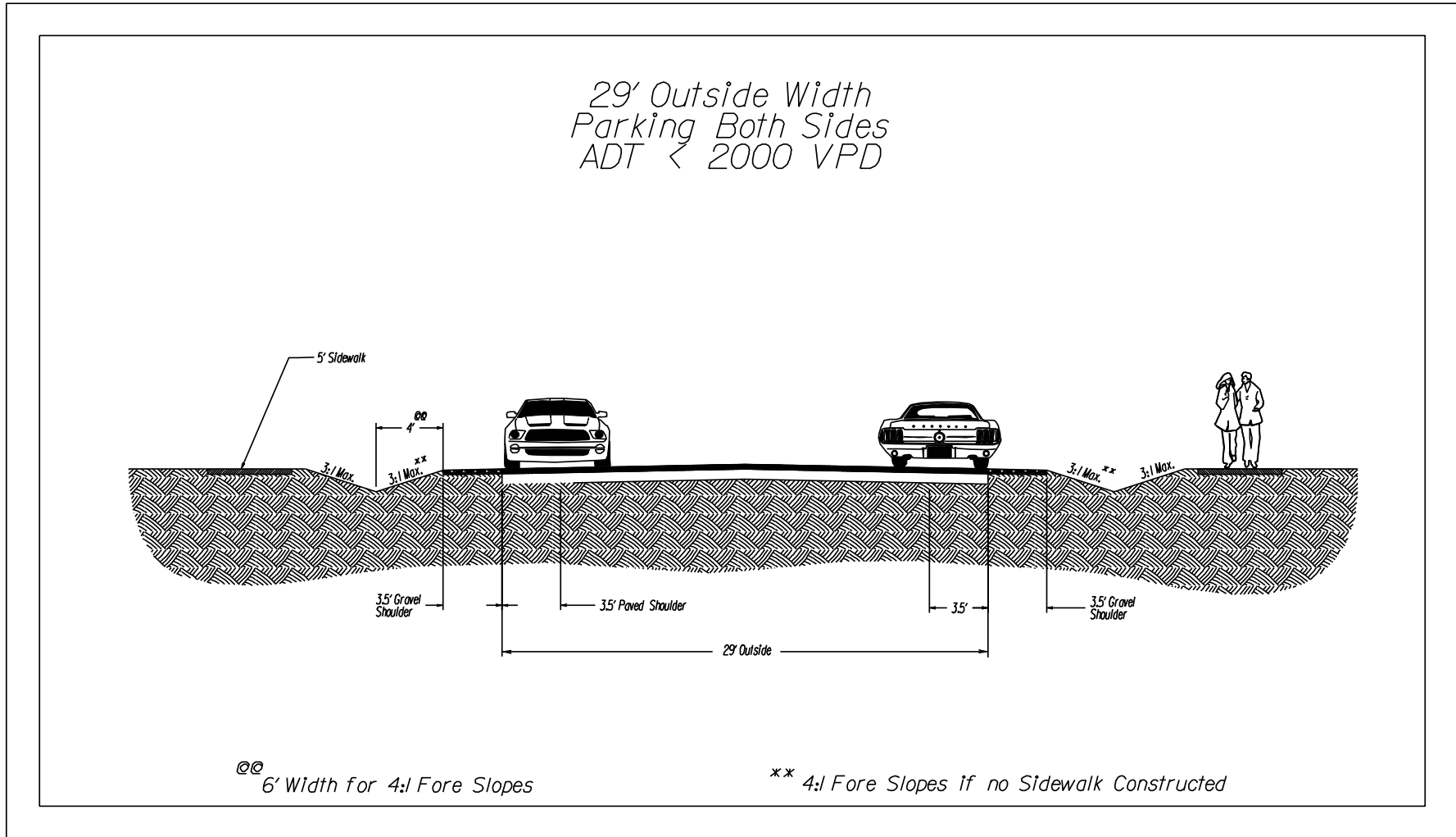
FIGURE 1.6 – 29' OUTSIDE WIDTH PARKING ON BOTH SIDES*
