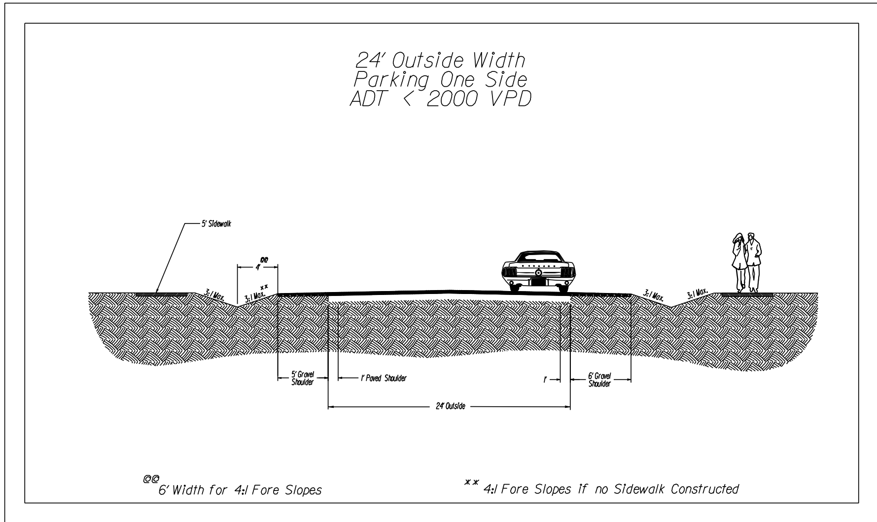
FIGURE 1.5 – 24' OUTSIDE WIDTH PARKING ONE SIDE*
