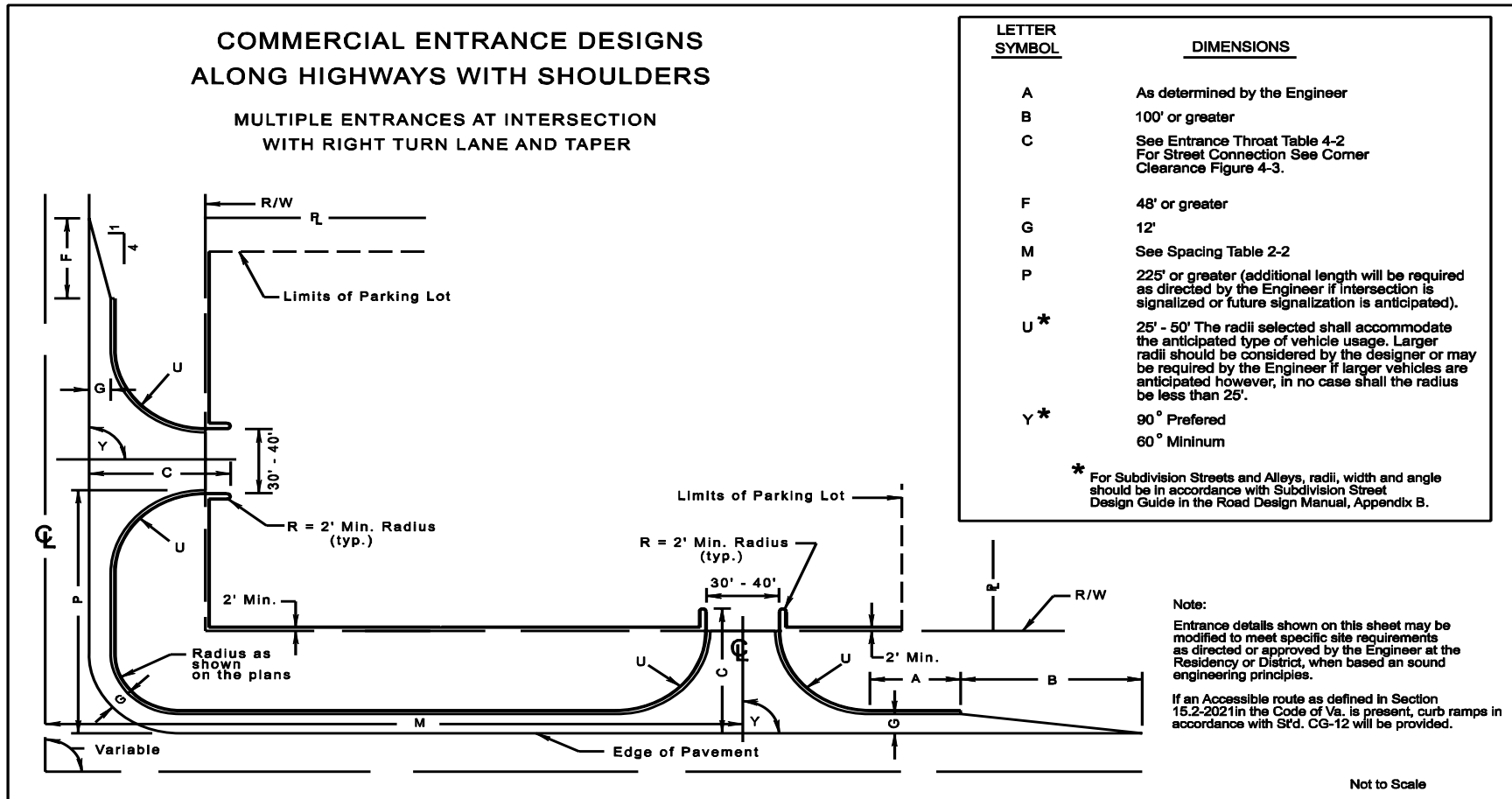
FIGURE 4-11 COMMERCIAL ENTRANCE DESIGNS ALONG HIGHWAYS WITH SHOULDERS AT INTERSECTION
