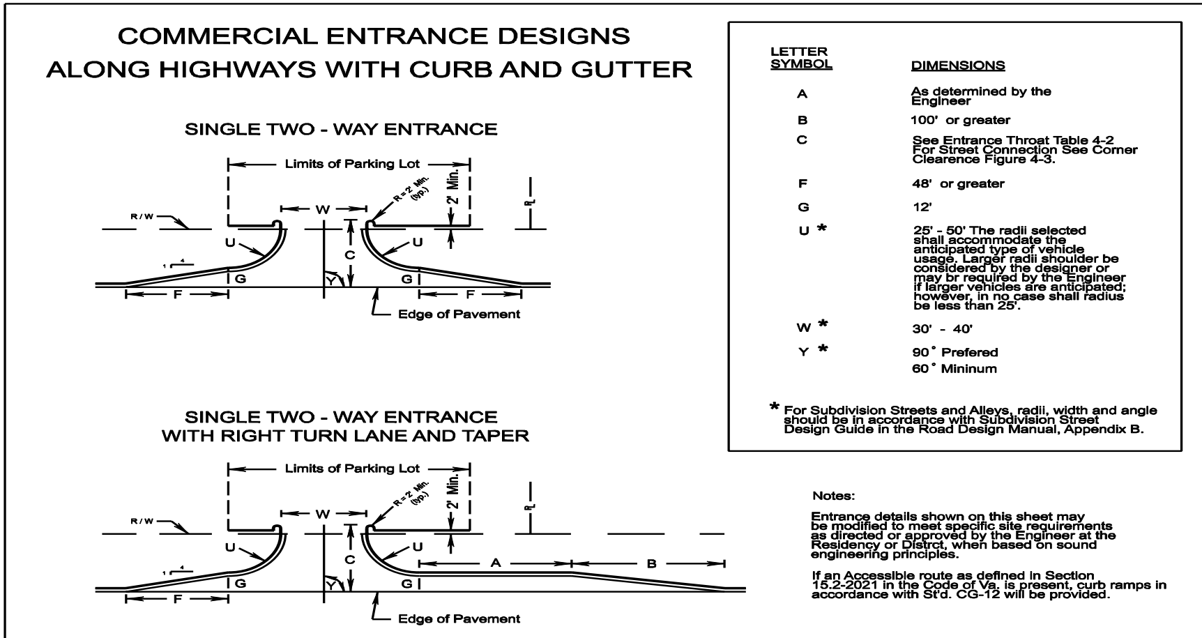
FIGURE 4-10 COMMERCIAL ENTRANCE DESIGNS ALONG HIGHWAYS WITH CURB AND GUTTER
