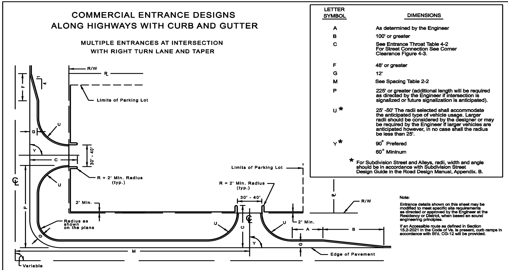
FIGURE 4-12 COMMERCIAL ENTRANCE DESIGNS ALONG HIGHWAYS WITH CURB AND GUTTER AT INTERSECTION
