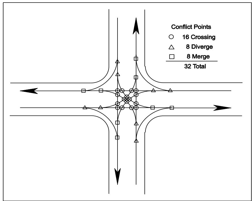
FIGURE 2-1 CONFLICT POINTS
