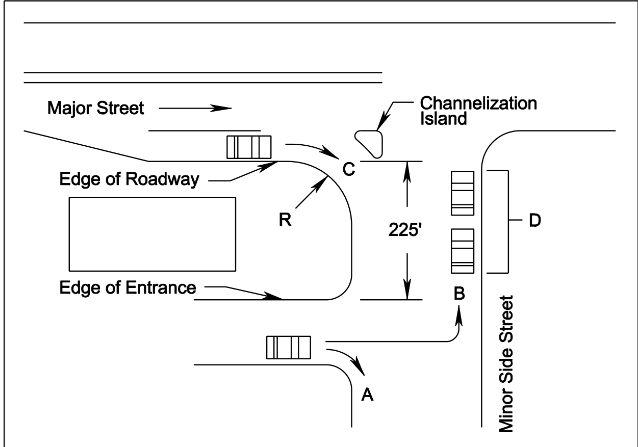
FIGURE 4-3 DOWNSTREAM CORNER CLEARANCE
