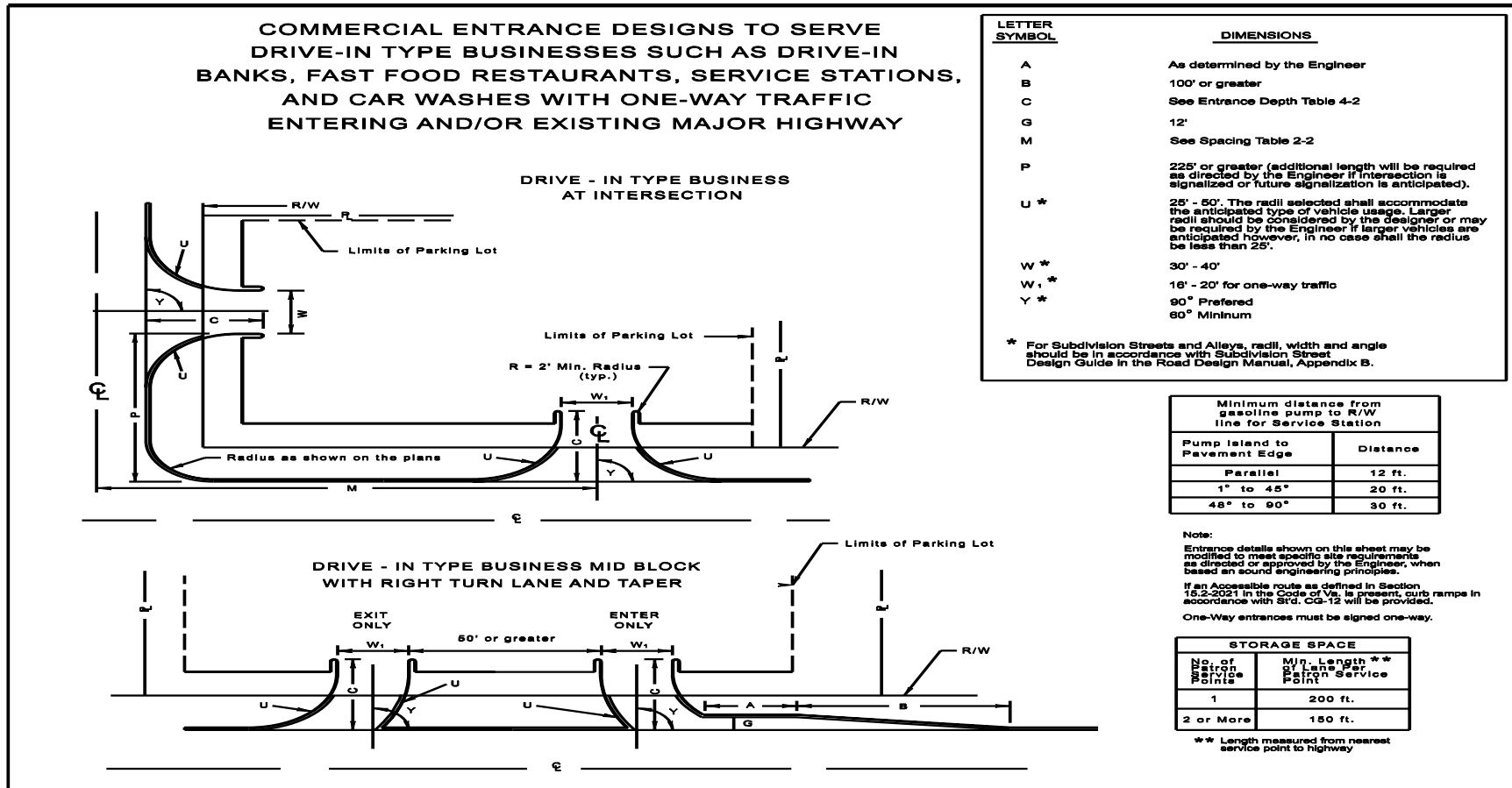
FIGURE 4-13 COMMERCIAL ENTRANCE DESIGNS ALONG HIGHWAYS WITH SHOULDERS
