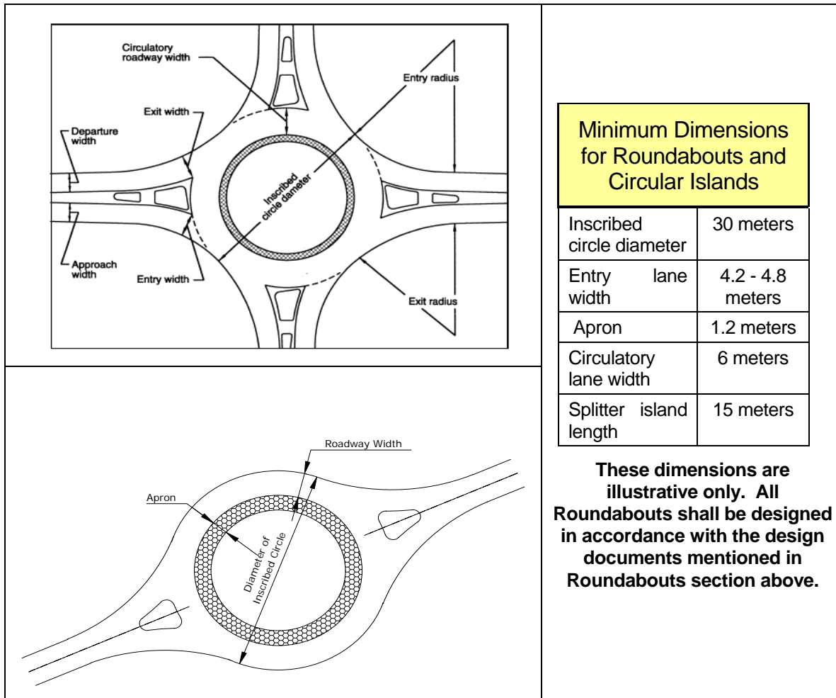
FIGURE C-1-2.2M ROUNDABOUT DETAILS
