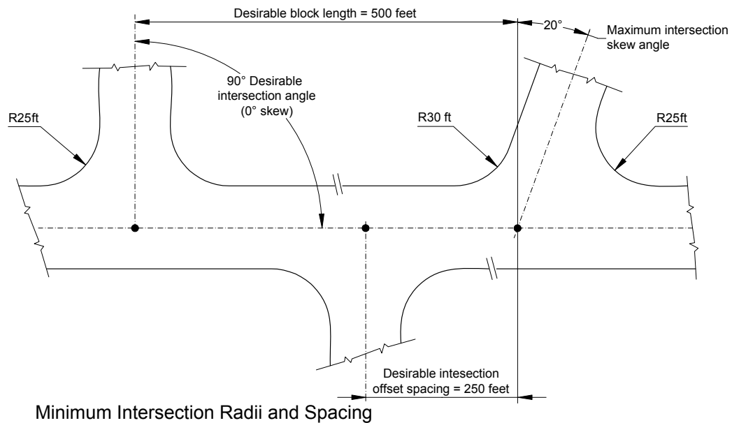
FIGURE 3 – INTERSECTION DESIGN
