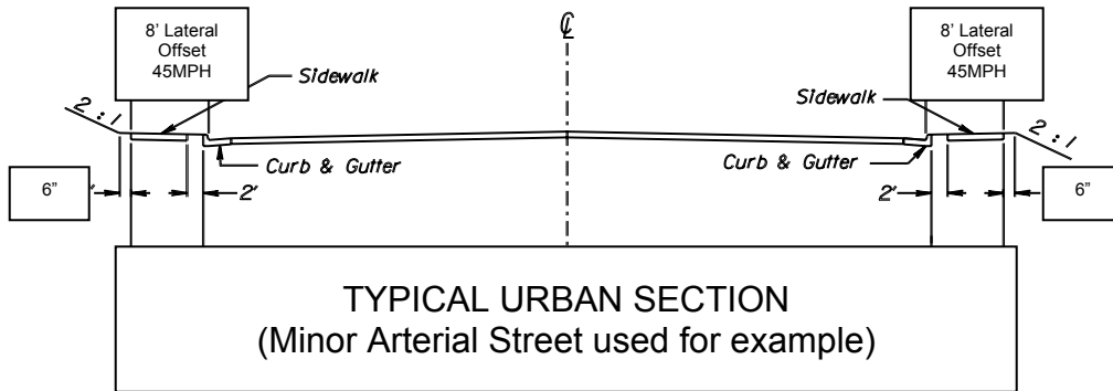
TYPICAL METHOD OF SHOWING CLEAR ZONE DATA ON TYPICAL SECTIONS
