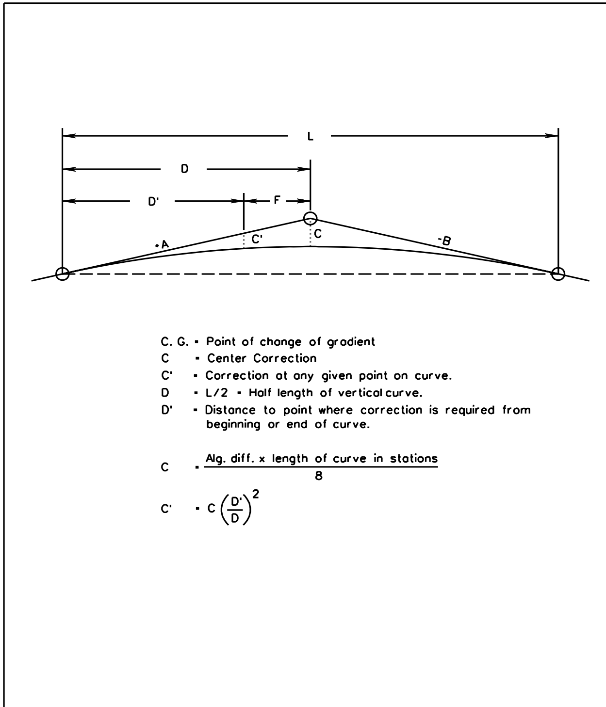
FIGURE C-6-9 PARABOLIC VERTICAL CURVE COMPUTATIONS*
