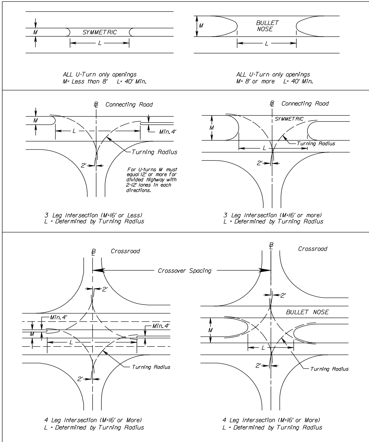
FIGURE C-1-3 CROSSOVERS WITH AND WITHOUT CONNECTIONS*
