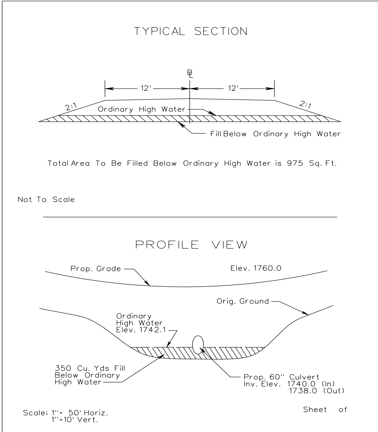
FIGURE C-4-7 CULVERT (NON-TIDAL) -TYPICAL SECTION AND PROFILE VIEW
