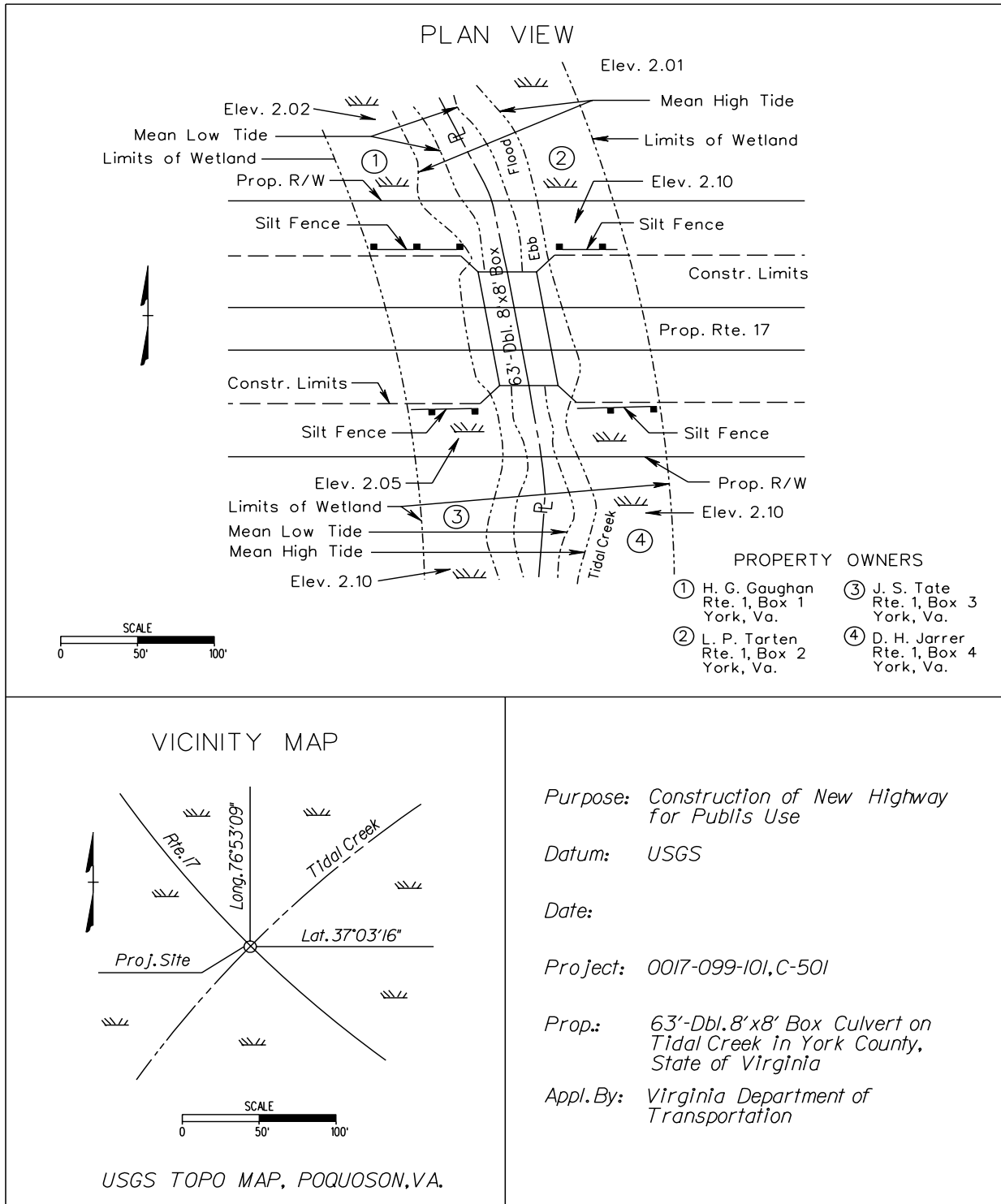
FIGURE C-4-8 CULVERT (TIDAL)-PLAN VIEW
