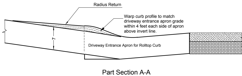
FIGURE 8 ROLLTOP CURB ENTRANCE DETAIL SECTION
