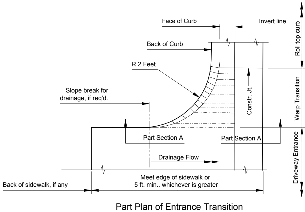
FIGURE 7 - ROLL TOP CURB ENTRANCE DETAIL
