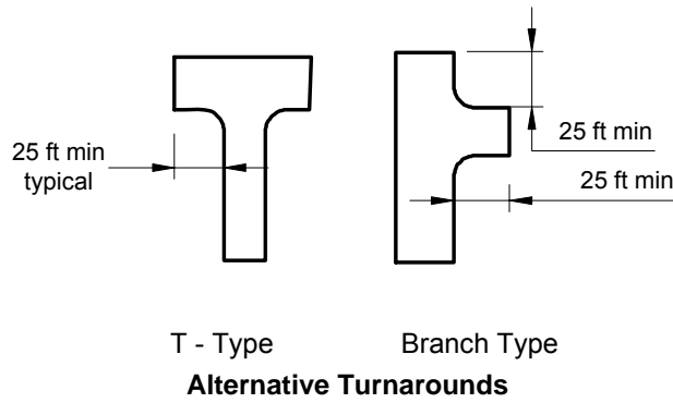
FIGURE 4 – CUL-DE-SAC DETAILS
