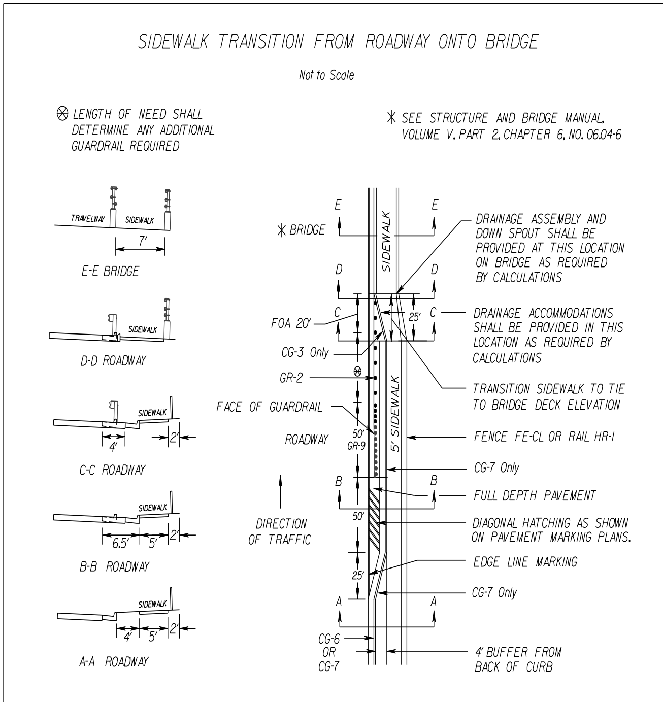
FIGURE A-5-12 SIDEWALK TRANSITION FROM ROADWAY ONTO BRIDGE FOR DESIGN SPEEDS >45 MPH*
