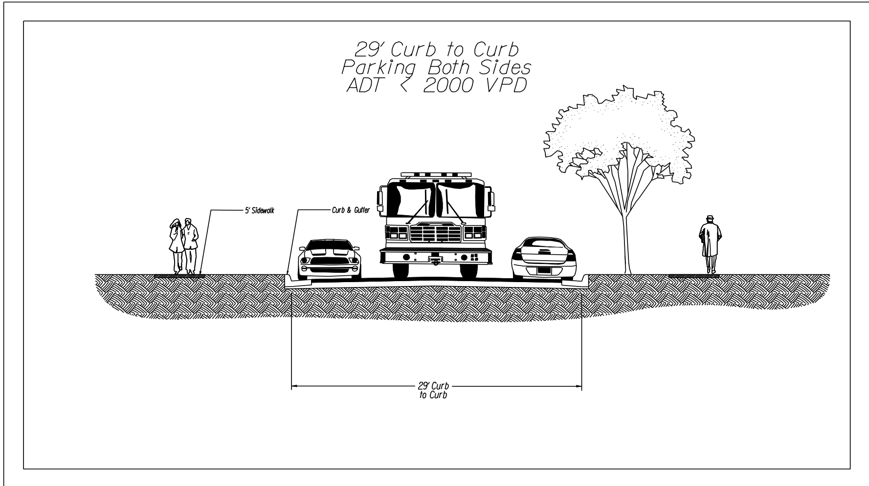
FIGURE 1.7 – 29' CURB TO CURB PARKING ON BOTH SIDES*
