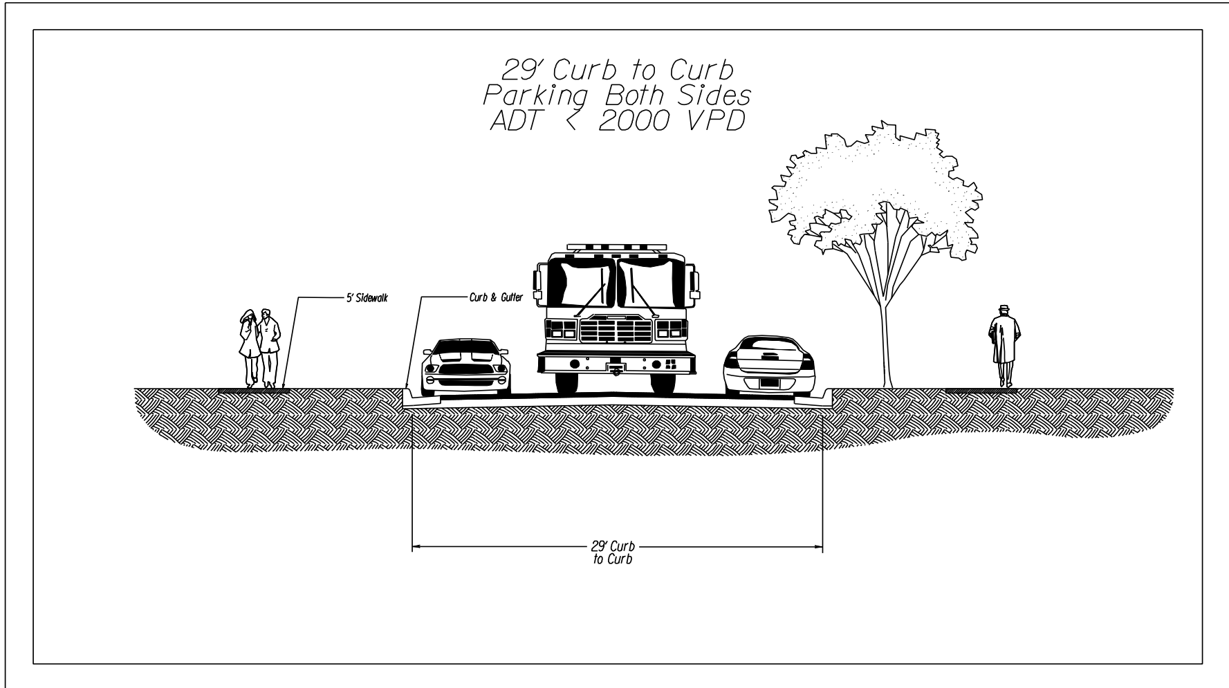
FIGURE 1.4 – 29' CURB TO CURB PARKING ON BOTH SIDES*
